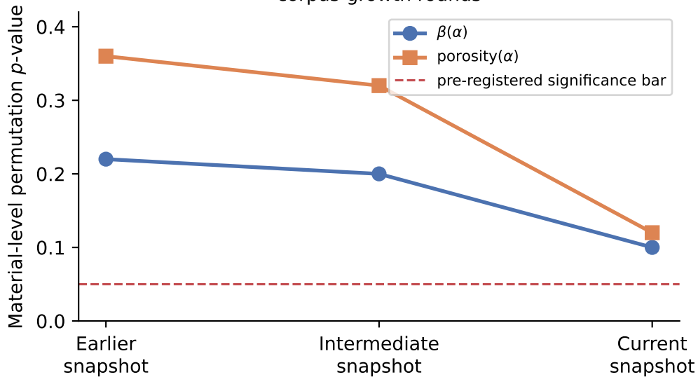
Permutation-test p -value across successive corpus-growth rounds
