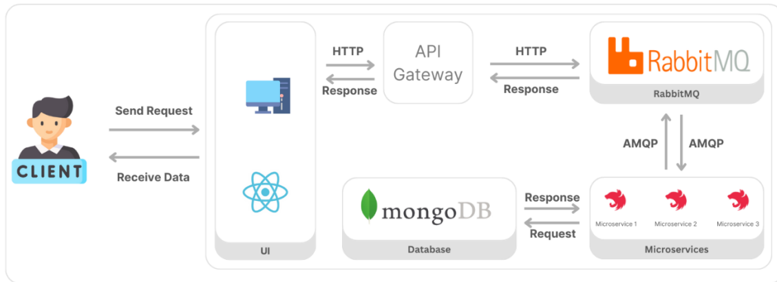
Figure 16 :Architecture microservice
