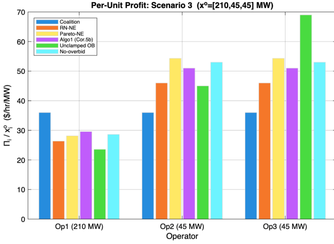
Fig. 12. Per-unit profit \Pi_i/x_i^o under Scenario 3. Algorithm 1 restores per-unit equity comparable to the Coalition benchmark.
