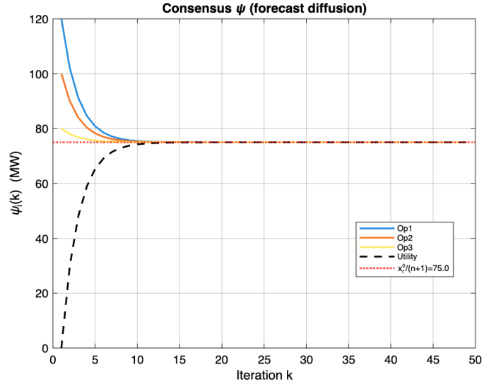
Fig. 14. Algorithm 1 consensus trajectory for \psi_i .
