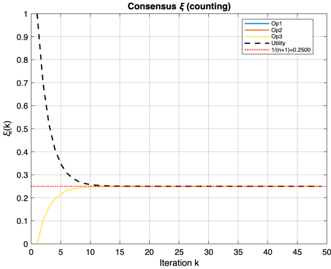
Fig. 13. Algorithm 1 consensus trajectory for \xi_i .
