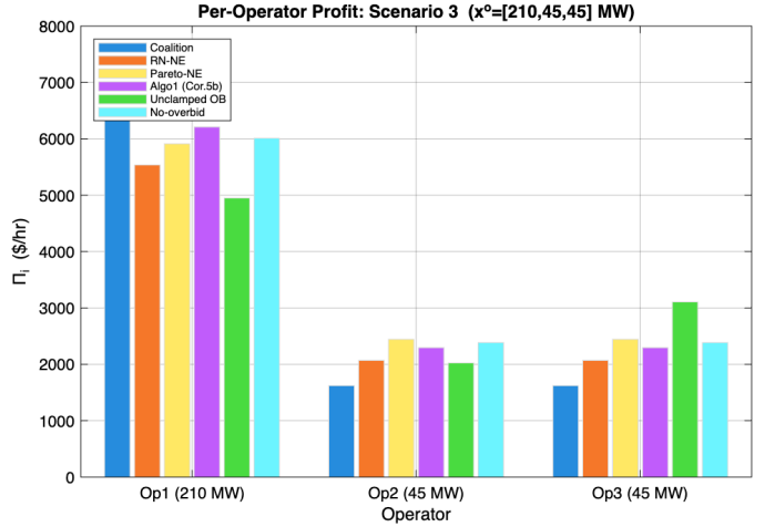
Fig. 11. Per-operator profit \Pi_i under Scenario 3 for all six strategies. Coalition and Algo 1 both achieve \sum \Pi_i = 10,800 $/hr at f = 0.5 ; risk-neutral and unclamped strategies reduce aggregate efficiency.
