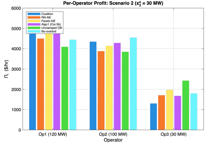
Fig. 7. Per-operator profit \Pi_i under Scenario 2 for all six strategies. Coalition and Algo 1 achieve the same total profit at f = 0.5 ; risk-neutral and unclamped strategies overshoot f = \frac{1}{2} , reducing aggregate efficiency.
