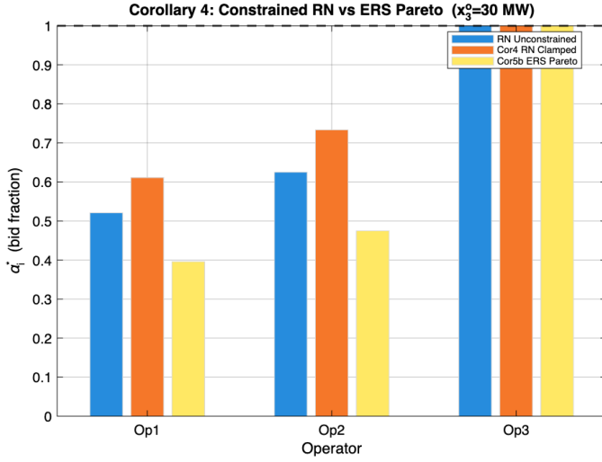
Fig. 9. Corollary 4: bidding strategies under unconstrained RN and constrained RN (Cor. 4 clamped) for Scenario 2 ( x_3^o = 30 MW). Constrained RN enforces feasibility but leaves f = 0.707 \gg \frac{1}{2} , incurring a persistent efficiency loss relative to risk-seeking coordination.
