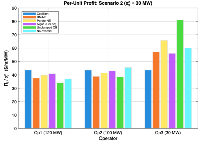
Fig. 8. Per-unit profit \Pi_i / x_i^o under Scenario 2. Algorithm 1 achieves per-unit equity comparable to the Coalition benchmark; unclamped overbidding distorts Op 3’s per-unit revenue upward at the expense of the other operators.
