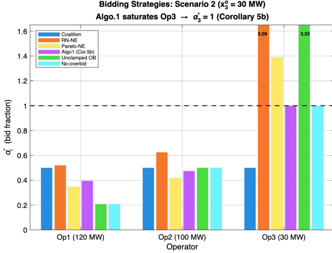
Fig. 6. Bidding strategies \alpha_i^* under Scenario 2 ( x_3^o = 30 MW). The dashed line marks \alpha = 1 ; both the unconstrained Pareto-NE and RN-NE overbid at Op 3, while Algorithm 1 (Corollary 5b saturation branch) places \alpha_3^* exactly at 1. Bars for RN-NE and Unclamped OB at Op 3 extend beyond the y -axis clip; their values are annotated.
