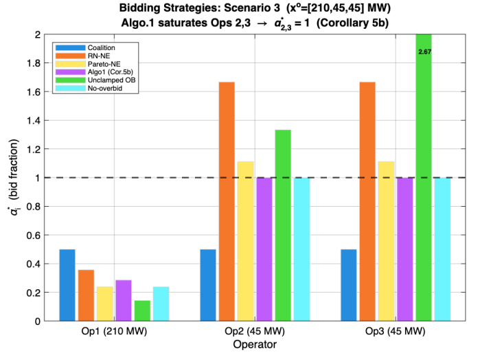
Fig. 10. Bidding strategies under Scenario 3 ( x^o = (210, 45, 45) MW). Both RN-NE and Pareto-NE overbid at Ops 2 and 3; Algorithm 1 (Cor. 5b) places \alpha_{2,3}^* exactly at 1. Naïve clamping reduces f below \frac{1}{2} .
