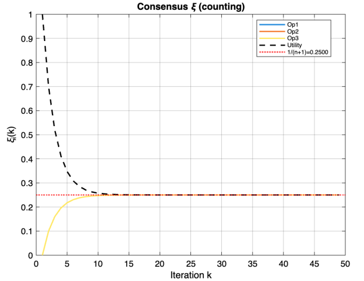
Fig. 12. Algorithm 1 consensus trajectory for \xi_i .
