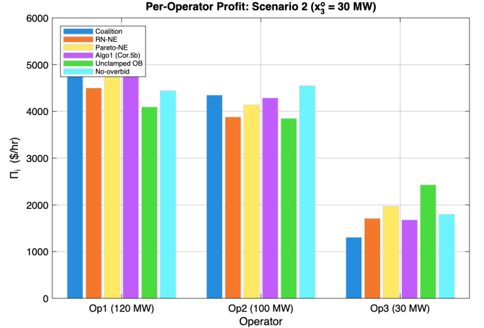
Fig. 9. Per-operator profit \Pi_i under Scenario 2 for all six strategies. Coalition and Algo 1 achieve the same total profit at f = 0.5 ; risk-neutral and unclamped strategies overshoot f = \frac{1}{2} , reducing aggregate efficiency.
