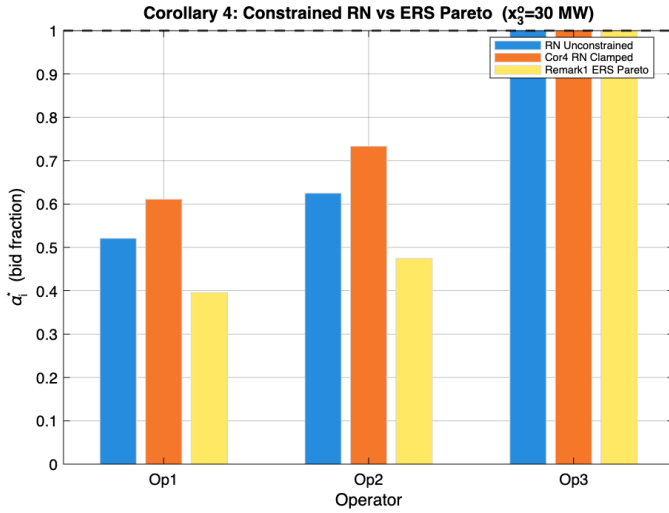
Fig. 11. Corollary 4: bidding strategies under unconstrained RN and constrained RN (Cor. 4 clamped) for Scenario 2 ( x_3^o = 30 \text{ MW} ). Constrained RN enforces feasibility but leaves f = 0.707 \gg \frac{1}{2} , incurring a persistent efficiency loss relative to risk-seeking coordination.
