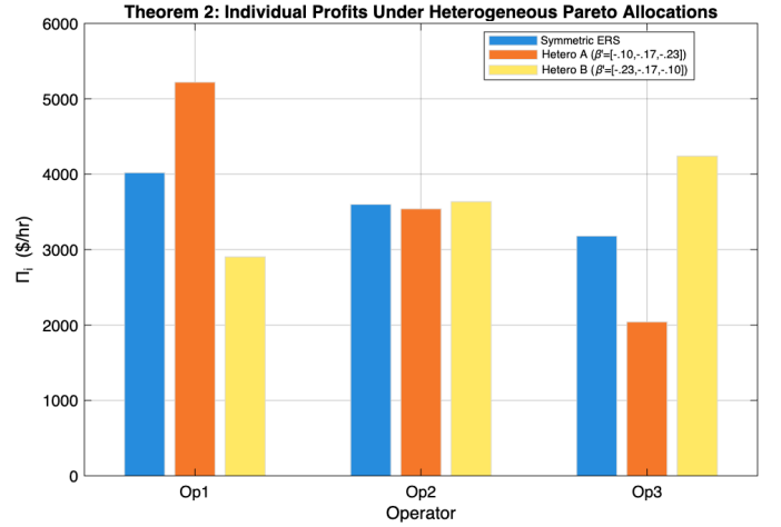
Fig. 7. Individual profits \Pi_i under the three allocations. Symmetric ERS and Hetero A achieve identical total profit but different per-operator splits.
