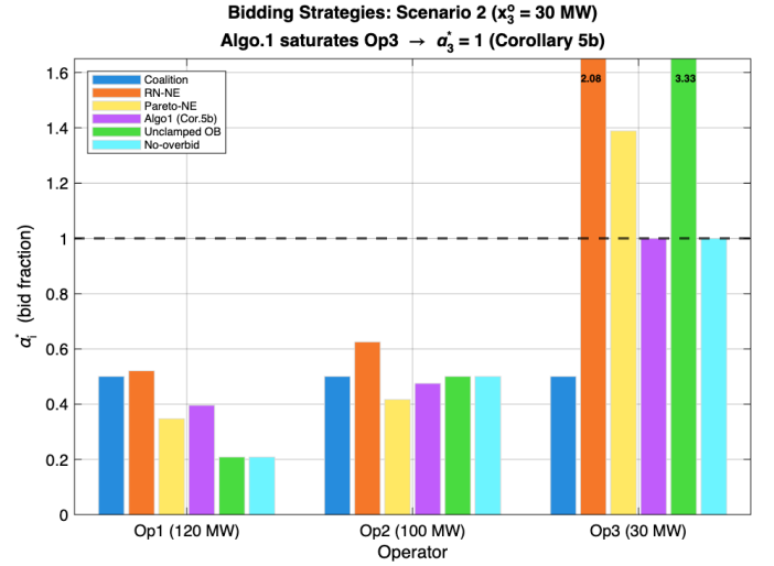
Fig. 8. Bidding strategies \alpha_i^* under Scenario 2 ( x_3^o = 30 \text{ MW} ). The dashed line marks \alpha = 1 ; both the unconstrained Pareto-NE and RN-NE overbid at Op 3, while Algorithm 1 (Corollary 5b saturation branch) places \alpha_3^* exactly at 1. Bars for RN-NE and Unclamped OB at Op 3 extend beyond the y -axis clip; their values are annotated.
