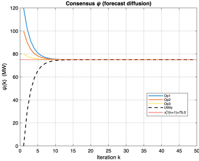
Fig. 13. Algorithm 1 consensus trajectory for \psi_i .
