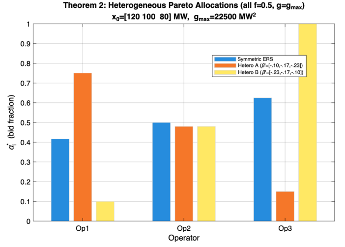
Fig. 6. Bidding strategies under three risk allocations all satisfying \sum \beta'_i = -\frac{1}{2} . Hetero B triggers overbidding at Op 3 and is infeasible without clamping.
