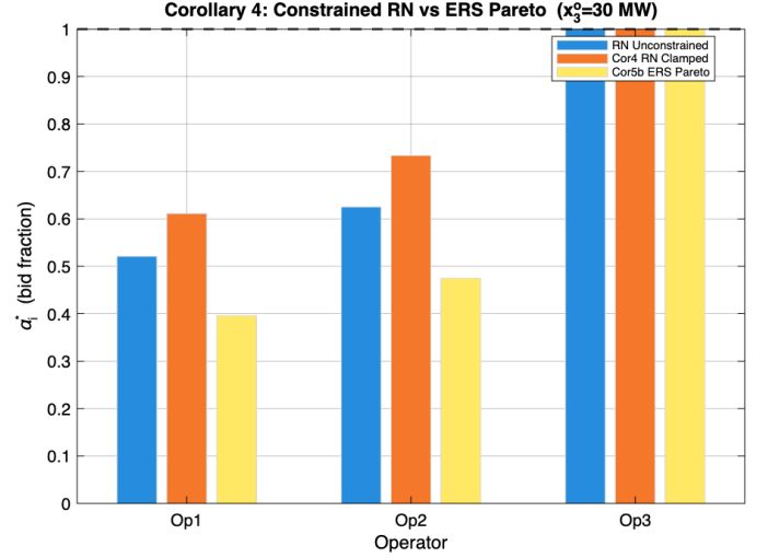
Fig. 9. Corollary 4: bidding strategies under unconstrained RN and constrained RN (Cor. 4 clamped) for Scenario 2 ( x_3^o = 30 MW). Constrained RN enforces feasibility but leaves f = 0.707 \gg \frac{1}{2} , incurring a persistent efficiency loss relative to risk-seeking coordination.
