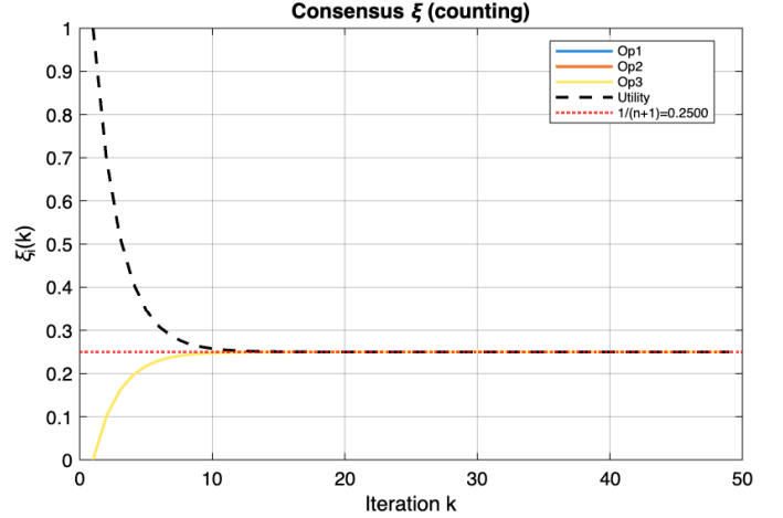
Fig. 13. Algorithm 1 consensus trajectory for \xi_i .
