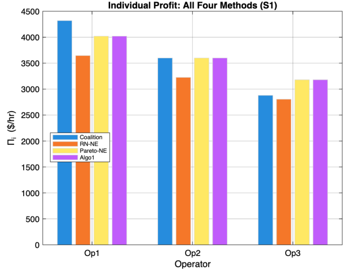
Fig. 4. Individual profits \Pi_i for all four strategies (Scenario 1).
