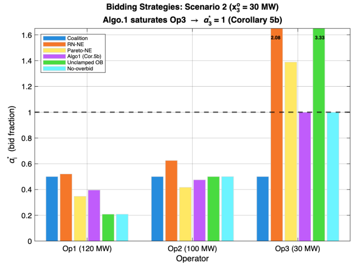
Fig. 6. Bidding strategies \alpha_i^* under Scenario 2 ( x_3^o = 30 \text{ MW} ). The dashed line marks \alpha = 1 ; both the unconstrained Pareto-NE and RN-NE overbid at Op 3, while Algorithm 1 (Corollary 5b saturation branch) places \alpha_3^* exactly at 1. Bars for RN-NE and Unclamped OB at Op 3 extend beyond the y -axis clip; their values are annotated.
