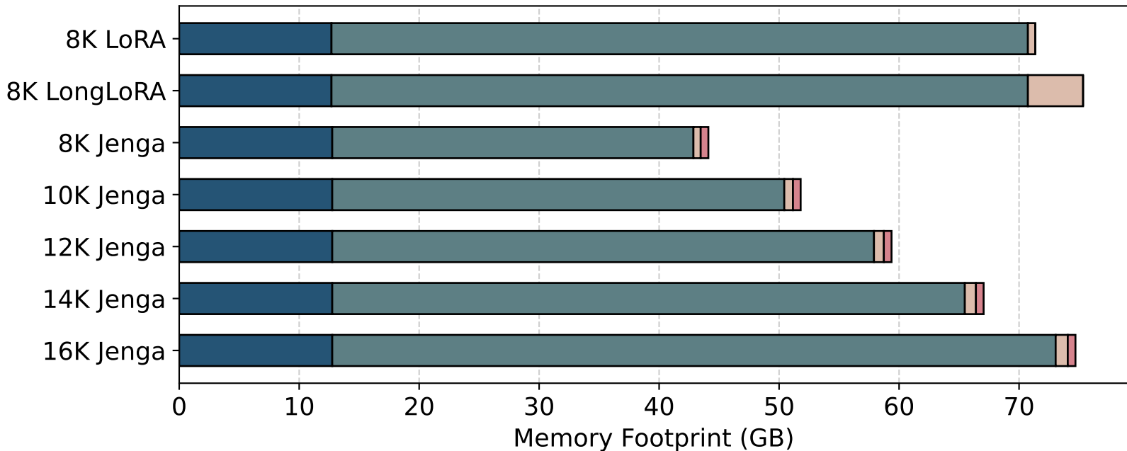
(a) Memory Footprint
