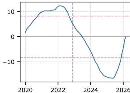
Mean Score
