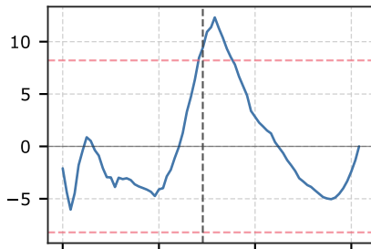
Answer Coverage
