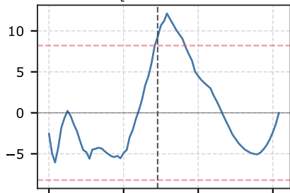
Accepted Rate
