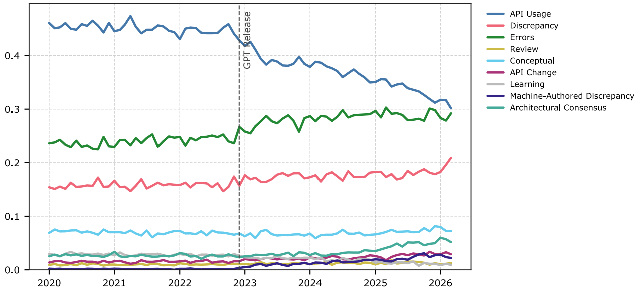
Fraction of Questions
