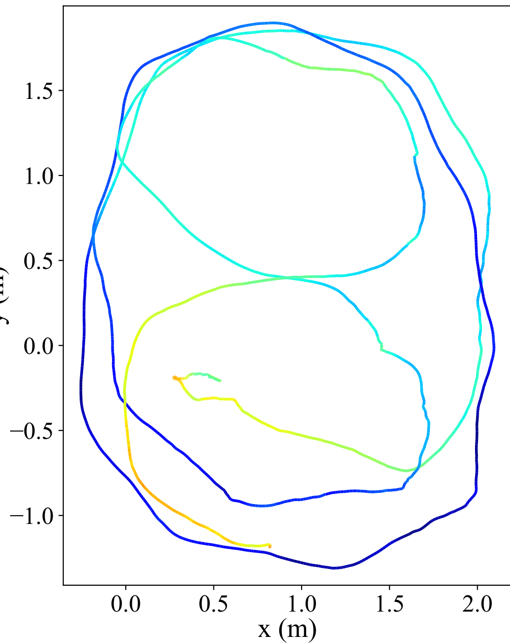
APE(m) of the proposed method
