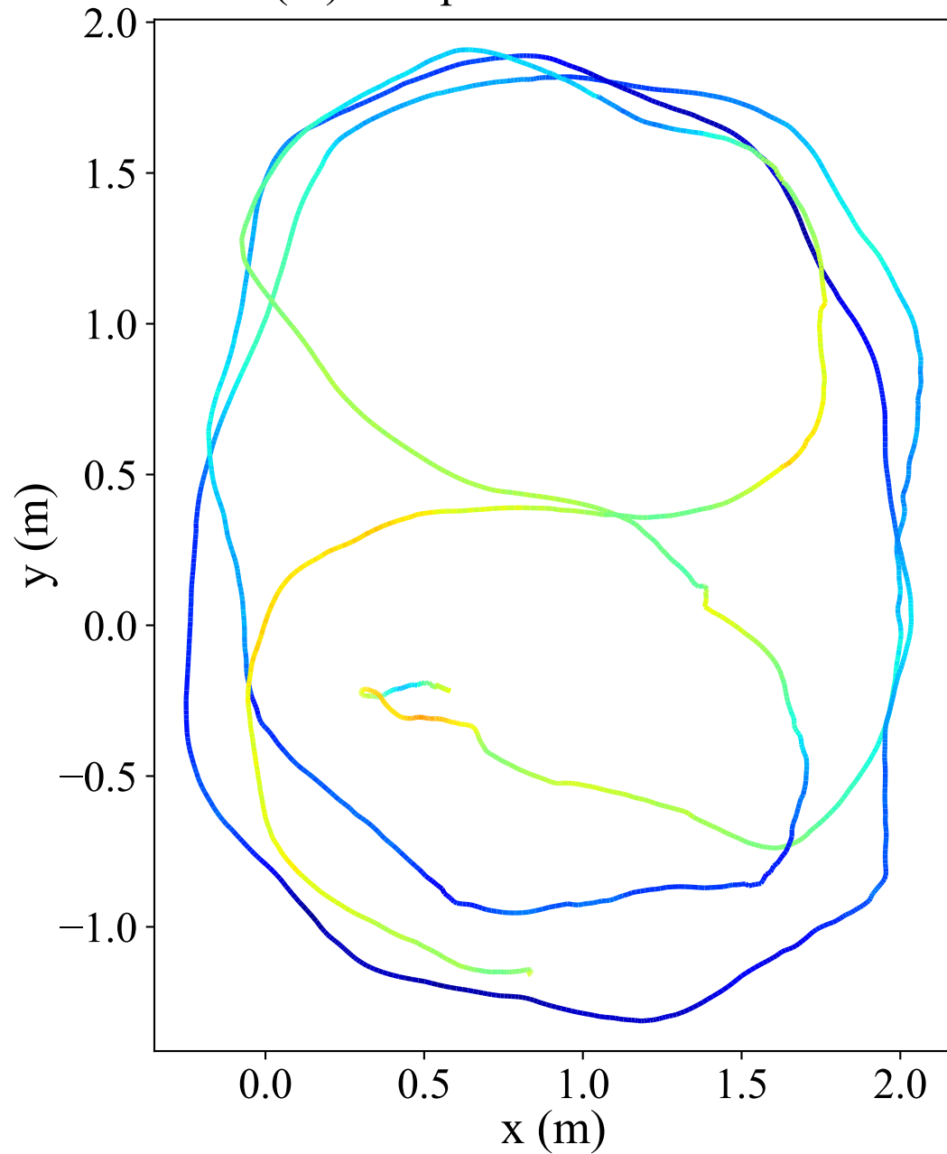
APE(m) of OpenVINS-Online method
