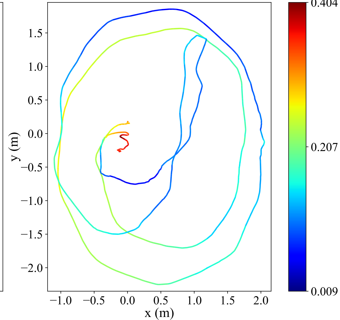
APE(m) of Kalibr method
