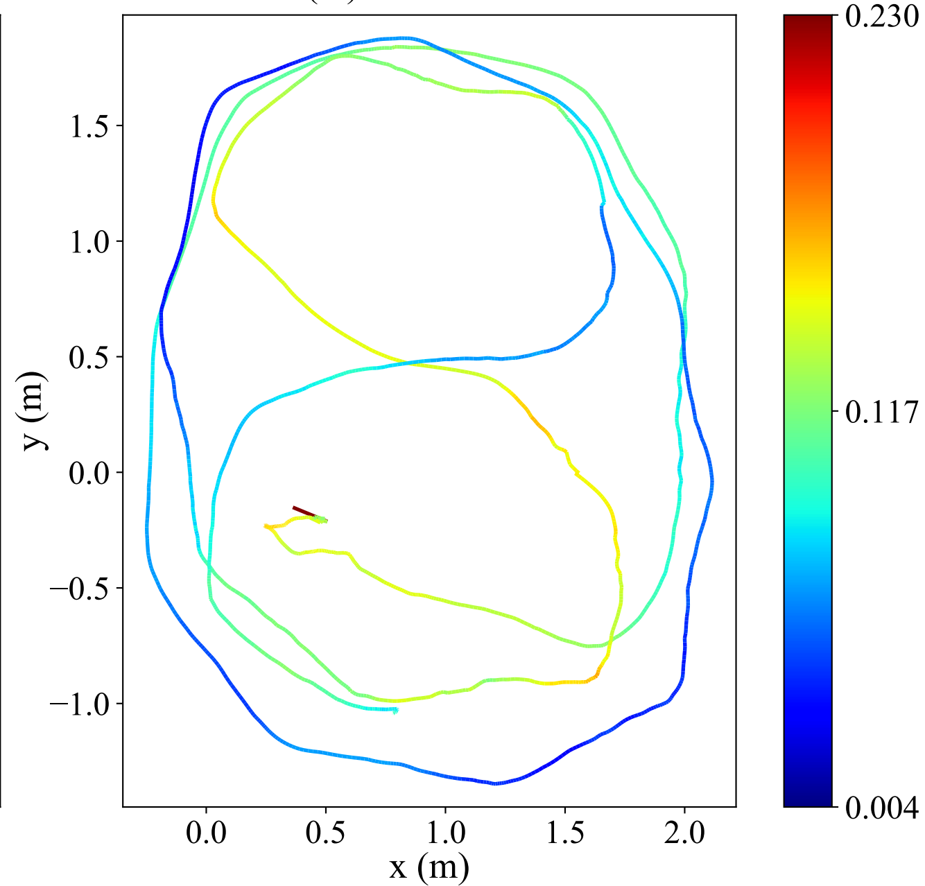
APE(m) of Kalibr method
