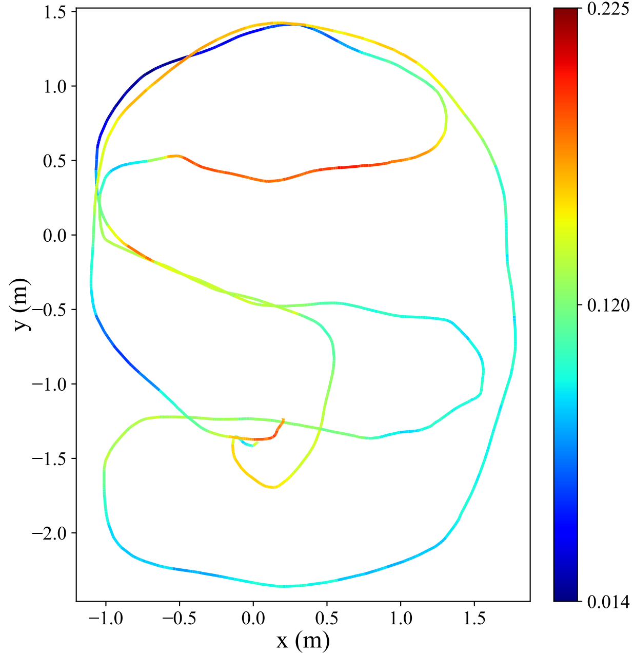
APE(m) of Kalibr method
