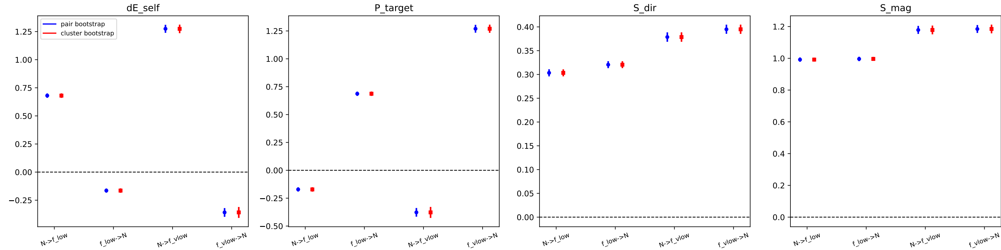
BOOT: pair-level vs cluster-level bootstrap 95% CI
