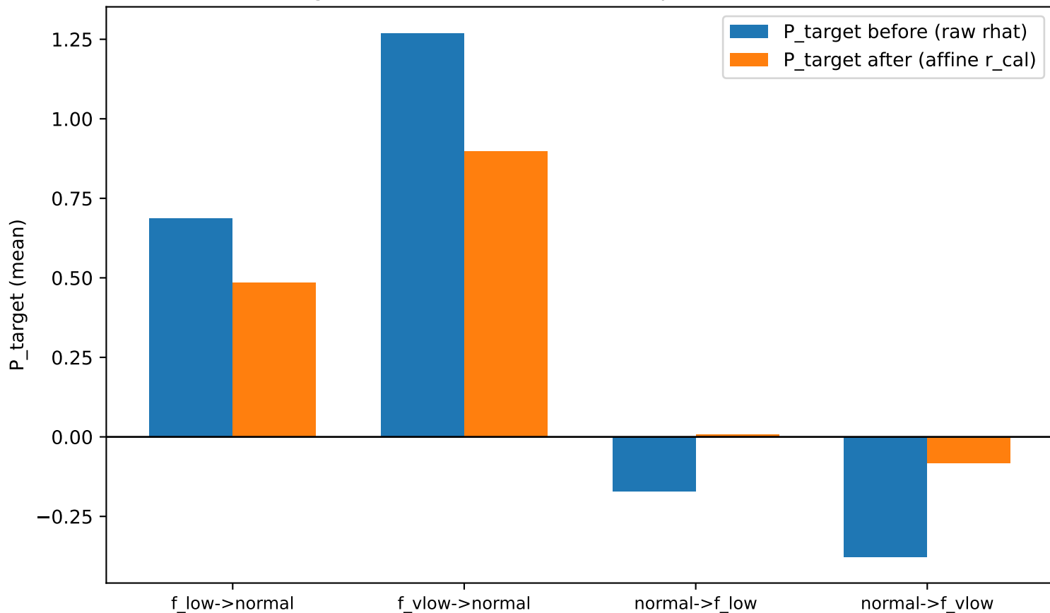
CAL: global affine calibration — swap metrics before/after
