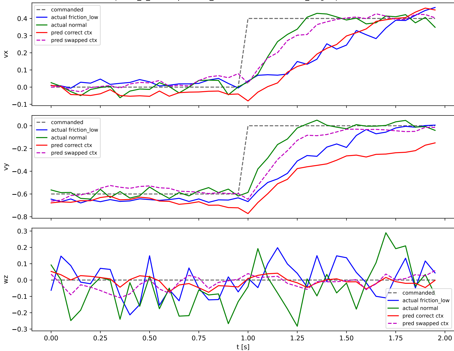
CS1: probe_4_lateral | friction_low->normal (median-P_target pair, P=0.757)
