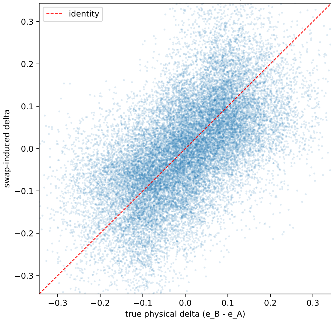
CS6: vx (corr=0.576, 24000 points)
