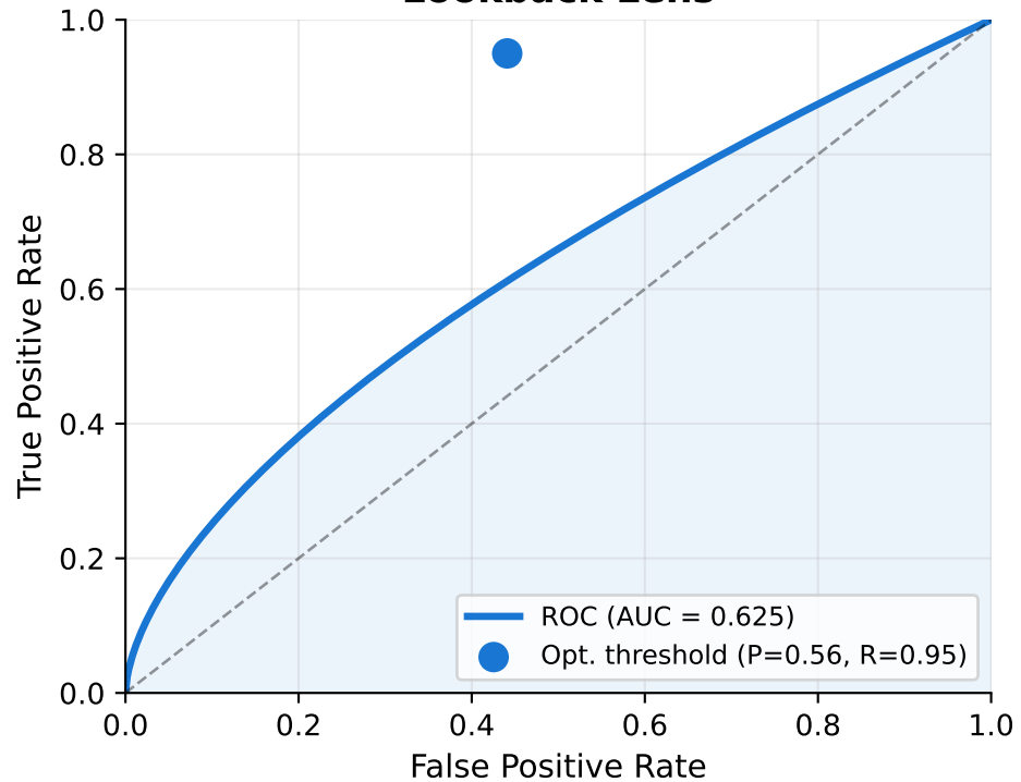
Lookback Lens
