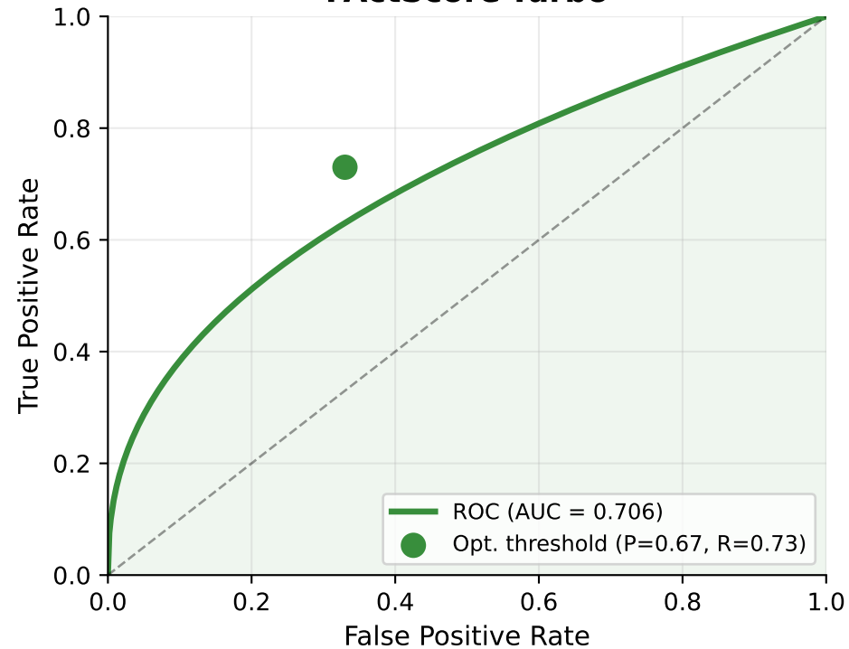
FactScore-Turbo
