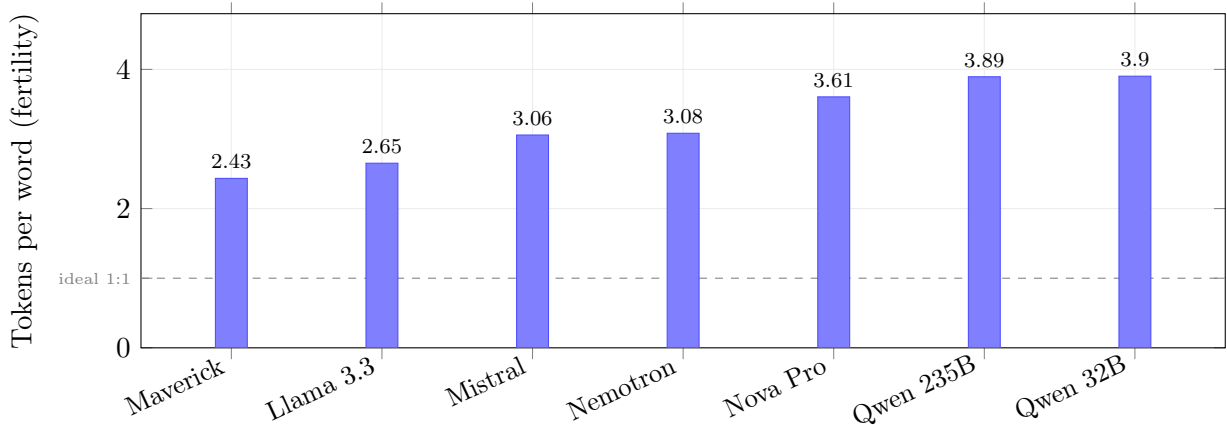
Figure 1: Tokenizer fertility (average tokens per whitespace-delimited word) on 100 Ukrainian legal documents. Lower is more efficient. Llama 4 Maverick produces 38% fewer tokens than Qwen3 on identical text (2.43 vs. 3.90 tokens/word); equivalently, Qwen3 consumes 60% more tokens than Maverick.
