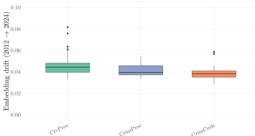
Рис. 9: Semantic embedding drift (2012→2024) by legal code. For each article, we embed 50 citing case snippets per year using E5-large and measure centroid shift. Civil Procedure shows the highest drift, consistent with its steepest MRR decline.
