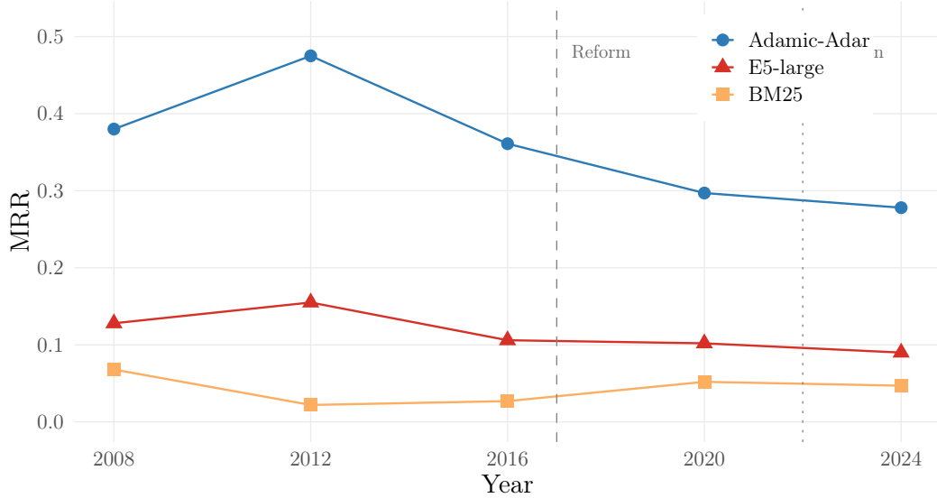
Рис. 3: MRR over time for three retrieval modalities. All three degrade; E5-large (dense) and Adamic-Adar (graph) decay at nearly identical rates (42% vs. 41%), while BM25 (lexical) decays 31%. Co-citation dominates in absolute terms ( \sim 3 \times E5).
