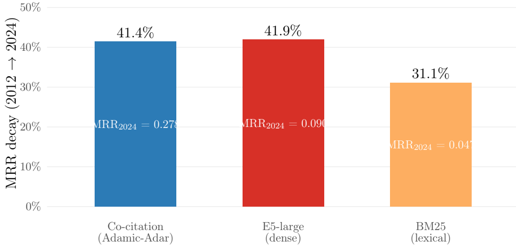
Рис. 4: Decay comparison (2012→2024). Dense retrieval does not escape temporal degradation. MRR 2024 values inside bars show absolute performance.
