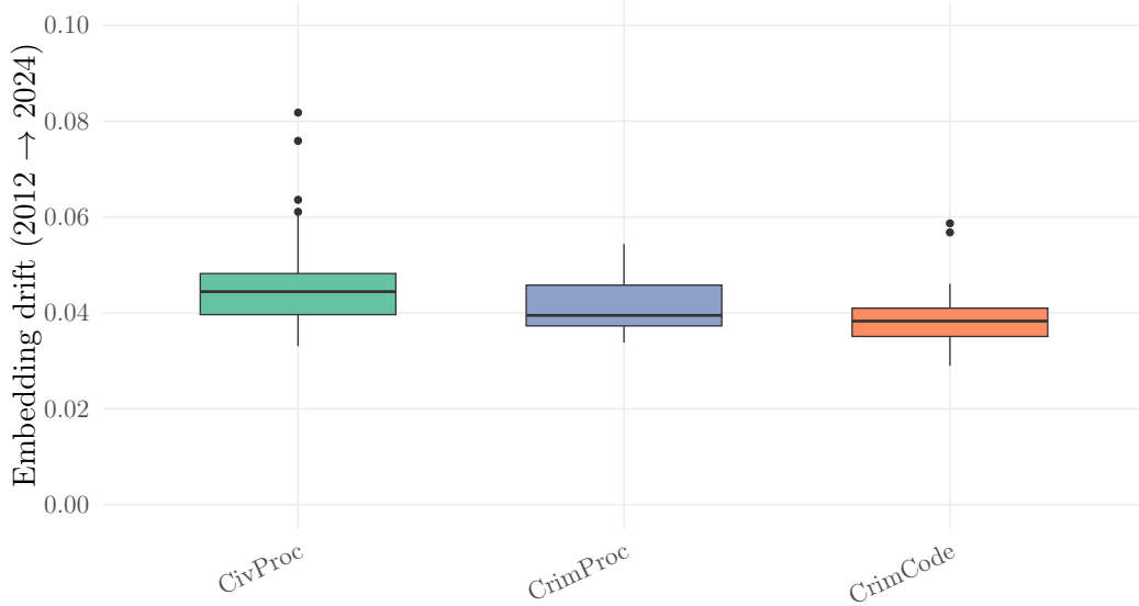
Рис. 9: Semantic embedding drift (2012→2024) by legal code. For each article, we embed 50 citing case snippets per year using E5-large and measure centroid shift. Civil Procedure shows the highest drift, consistent with its steepest MRR decline.
