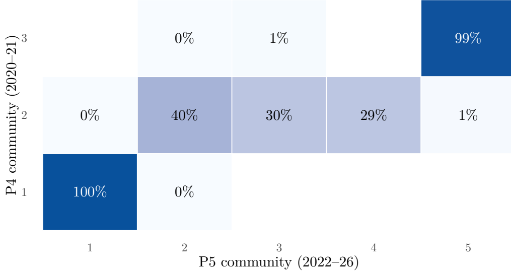
Figure 6: Transition matrix P4→P5. Cell values show percentage of P4 community assigned to each P5 community.
