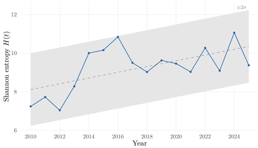
Figure 8: Shannon entropy (2010–2025). No year exceeds the \pm 2\sigma significance threshold.
