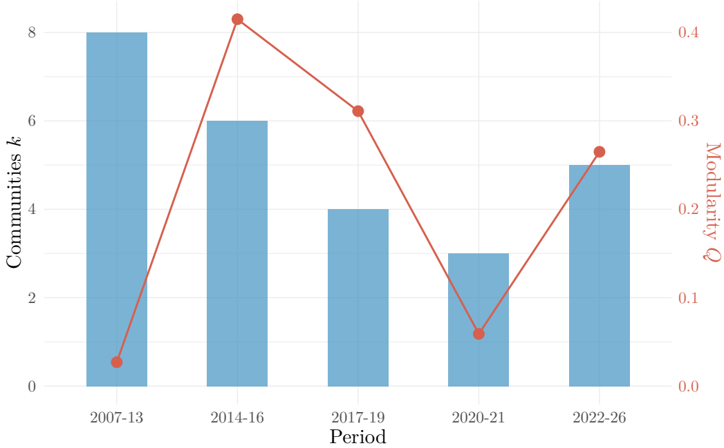
Figure 3: Community count k and modularity Q across periods. Effective k_{\text{eff}} = 4, 5, 4, 3, 5 (excluding P1 micro-clusters).
