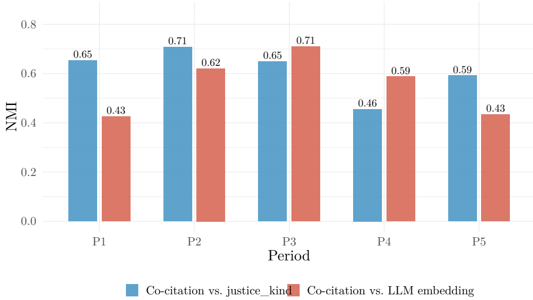
Figure 14: Comparison of two validation metrics per period: NMI between co-citation communities and formal jurisdiction (blue), and NMI between co-citation communities and LLM embedding clusters (red). The metrics align at P3 and diverge at P5, where co-citation captures practice-based distinctions invisible to semantics.
