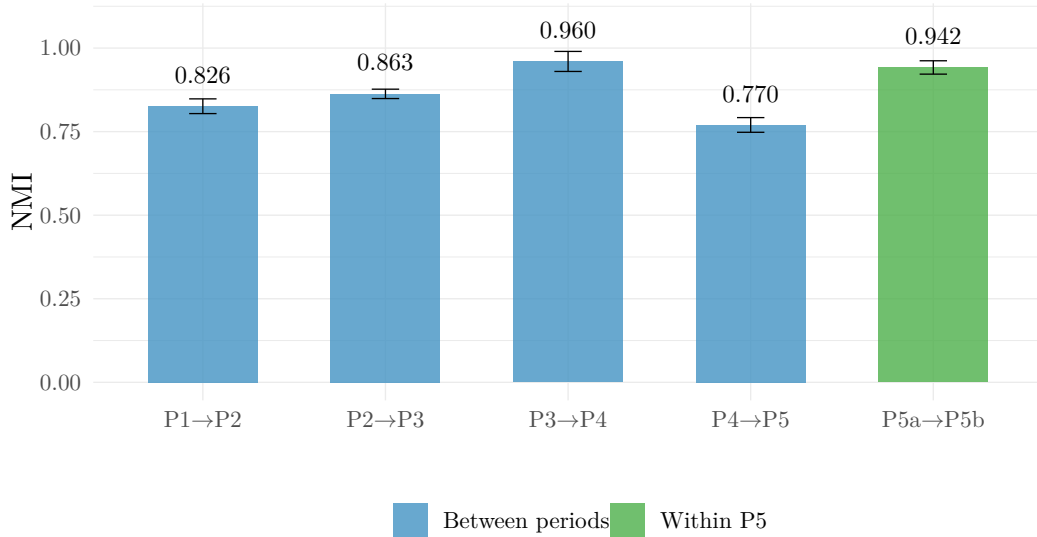
Figure 15: Extended NMI comparison including within-P5 stability (P5a→P5b, green). The wartime reorganization stabilizes rapidly (NMI = 0.942), contrasting with the P4→P5 disruption (NMI = 0.770).
