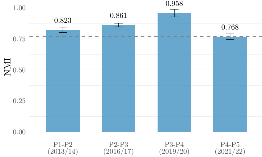
Figure 5: Bootstrapped NMI (error bars: \pm 2\sigma ). P4→P5 is the strongest shock; P3→P4 is near-perfect stability.
