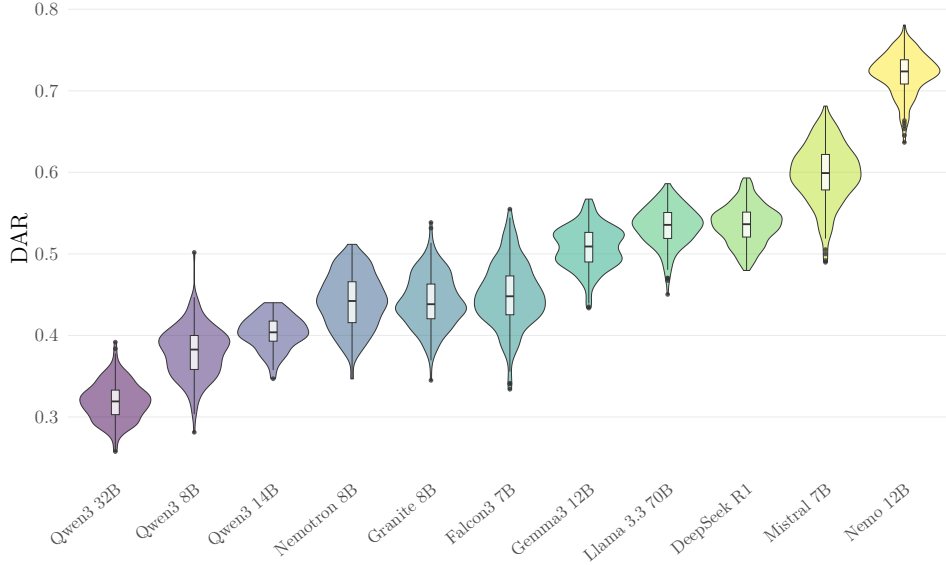
Figure 4: DAR distribution across 11 Transformer models. DAR does not predict few-shot benefit ( r = +0.02 ).
