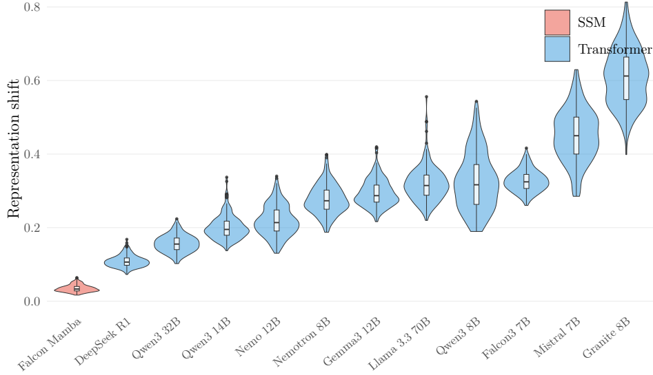
Figure 5: Representation shift: Falcon Mamba (SSM, red) vs. Transformers (blue).
