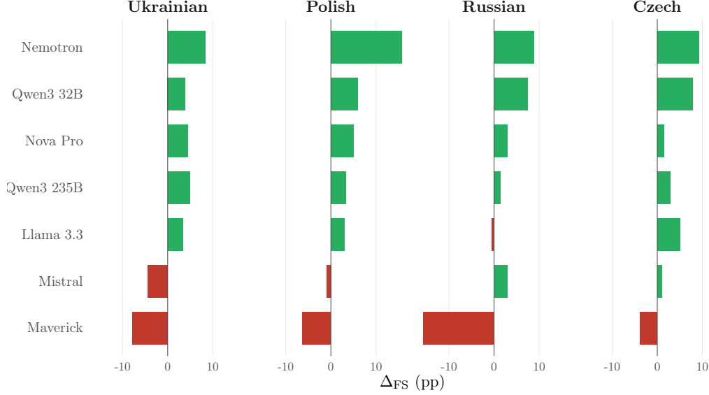
Figure 3: Few-shot delta ( \Delta_{\text{FS}} , pp) across four Slavic languages on SIB-200. Red bars = degradation, green = improvement. Maverick degrades on all four languages; Nemotron improves on all four. The pattern is model-intrinsic, not language-dependent.
