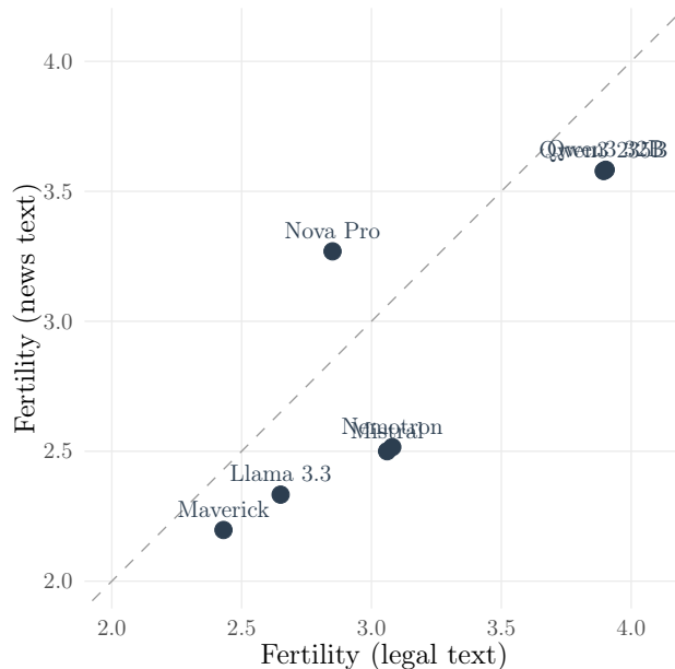
Figure 1: Cross-domain fertility: legal text (Ovcharov, 2026a) vs. news text (SIB-200). The dashed line marks y = x ; points below it indicate lower fertility on news. Model rankings are preserved (Spearman \rho = 0.89 ), confirming fertility is a tokenizer property. Nova Pro is the sole outlier above the diagonal.
