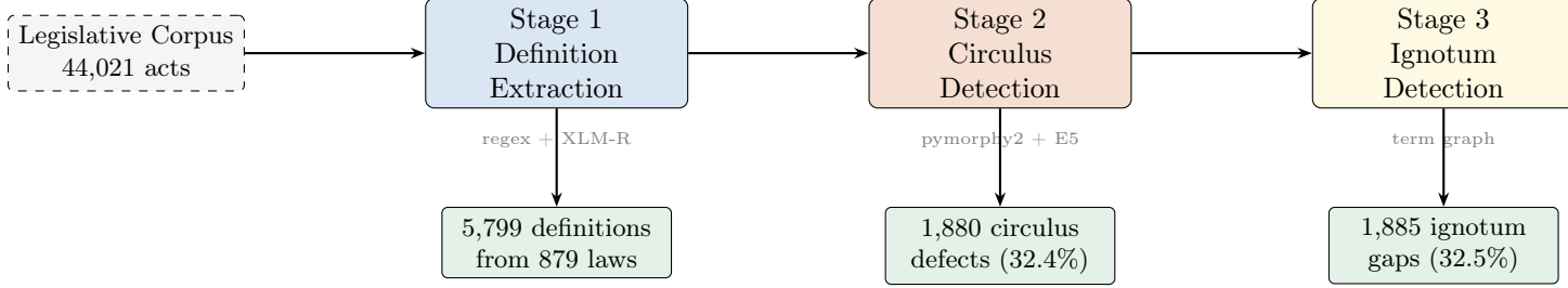
Рис. 1: The DefectRadar pipeline. Stage 1 extracts definitions from legislative text. Stage 2 detects circulus in definiendo via morphological and semantic analysis. Stage 3 constructs a cross-legislative definition graph to detect ignotum per ignotum.
