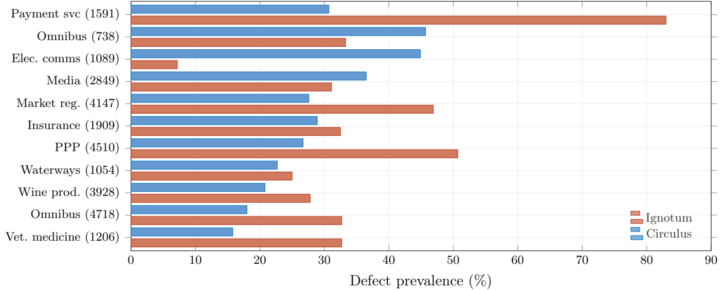
Рис. 3: Defect prevalence in the top-11 laws by definition count. Payment services law (1591-IX) exhibits the highest ignotum rate (83.0%), while electronic communications (1089-IX) has the highest circulus rate among single-domain laws (44.9%).
