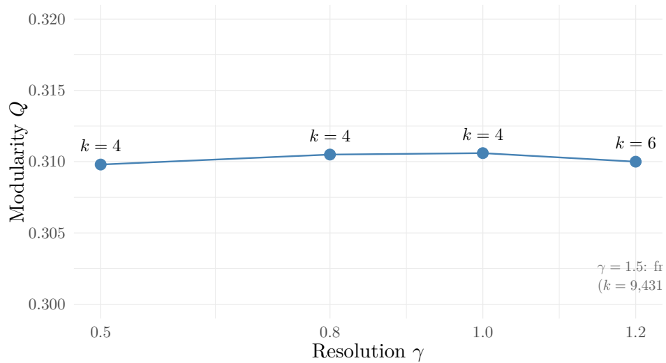
Figure 12: Resolution sensitivity on P3 (2017–2019). Community count and modularity are stable for \gamma \in [0.5, 1.2] ; only \gamma = 1.5 produces degenerate fragmentation.
