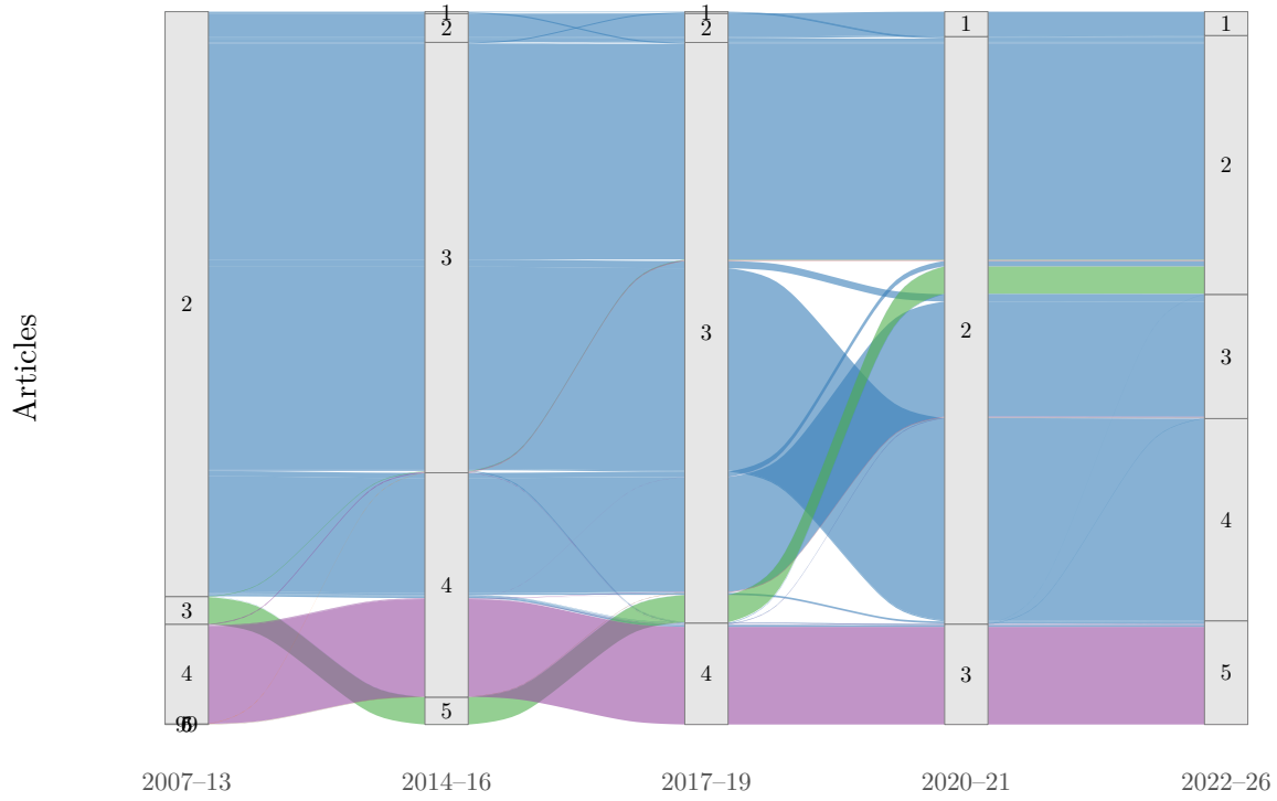
Figure 3: Community evolution across five periods (alluvial diagram, 6,666 core nodes present in all periods). Flow width indicates shared nodes between community assignments. Merging flows during P1–P4 show consolidation; splitting flows at P5 show wartime diversification.
