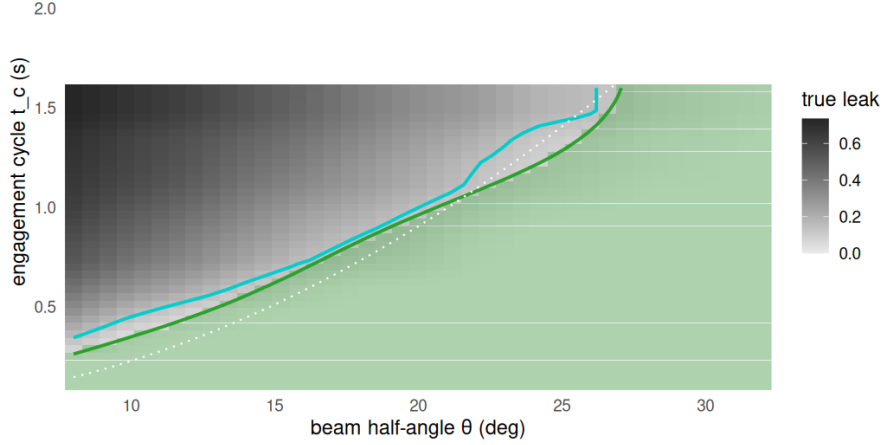
Figure 4: E3. The certified-safe envelope \hat{A} (green) sits conservatively inside the true safe region; the conformal boundary U = \tau (green) is a safe margin below the true boundary L = \tau (cyan), with no false-safe points.
