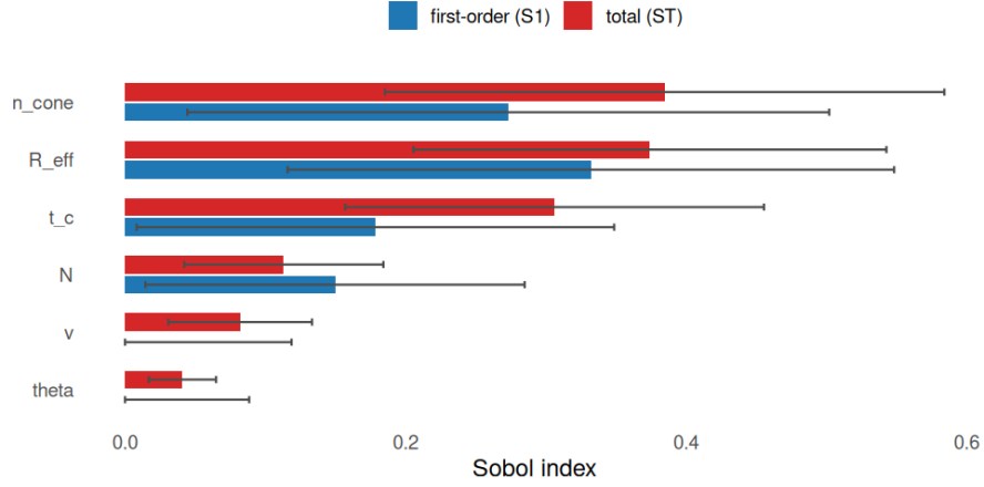
Figure 6: E5. Sobol first-order ( S_1 ) and total ( S_T ) indices with confidence intervals; n_{\text{cone}} and R_{\text{eff}} co-dominate the penetration variance.
