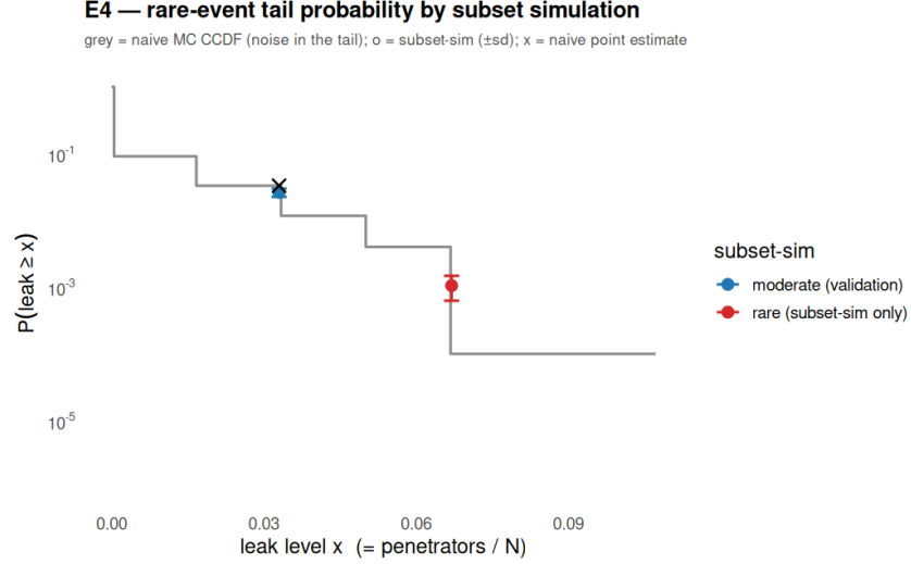
Figure 5: E4. Naive Monte-Carlo CCDF (grey) is pure noise in the tail; subset simulation (o, \pm sd) resolves the penetration probability where naive MC has a single sample (x).
