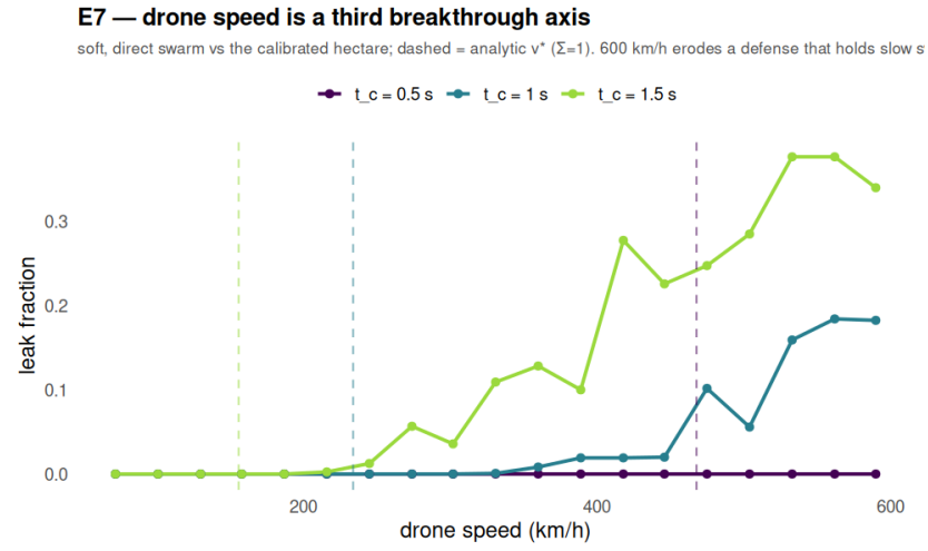
Figure 8: E7. Leak vs drone speed for three engagement cycles; a 600 km/h swarm penetrates a defense that holds slow swarms. Dashed: analytic single-aperture v^* (a lower bound).
