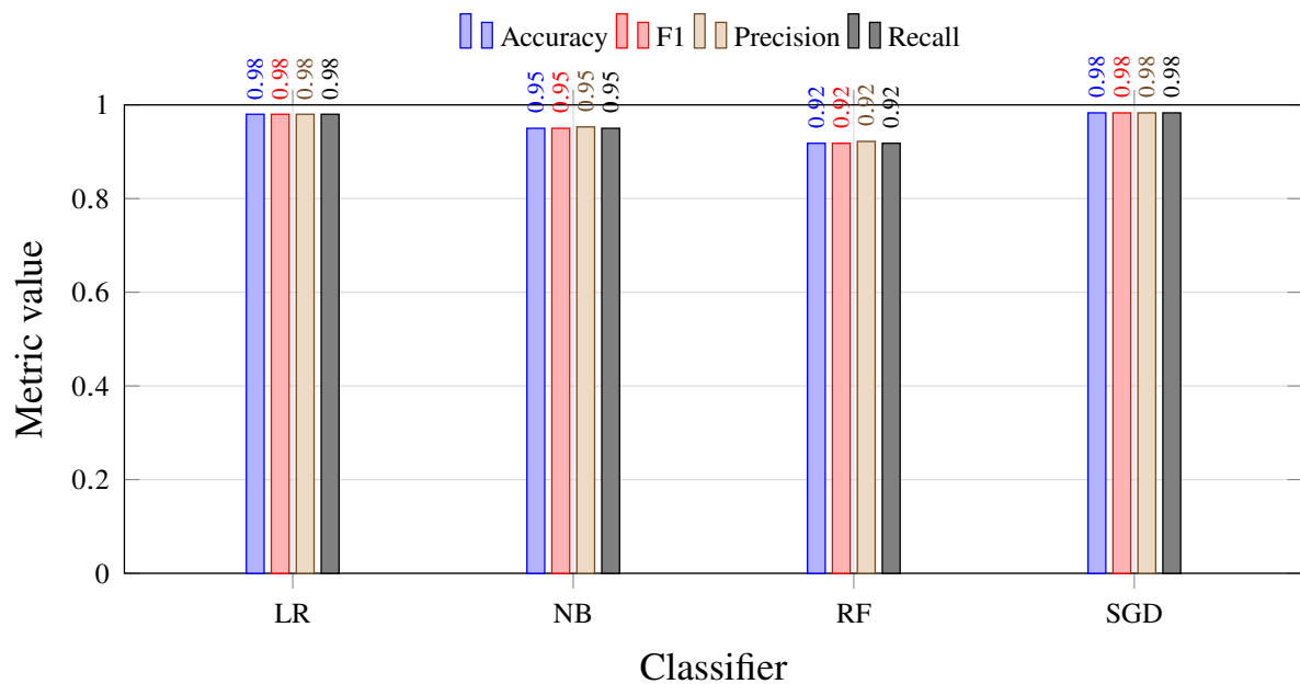
Fig. 4. Classifier comparison reconstructed from the checked-in ML evaluation plot.
