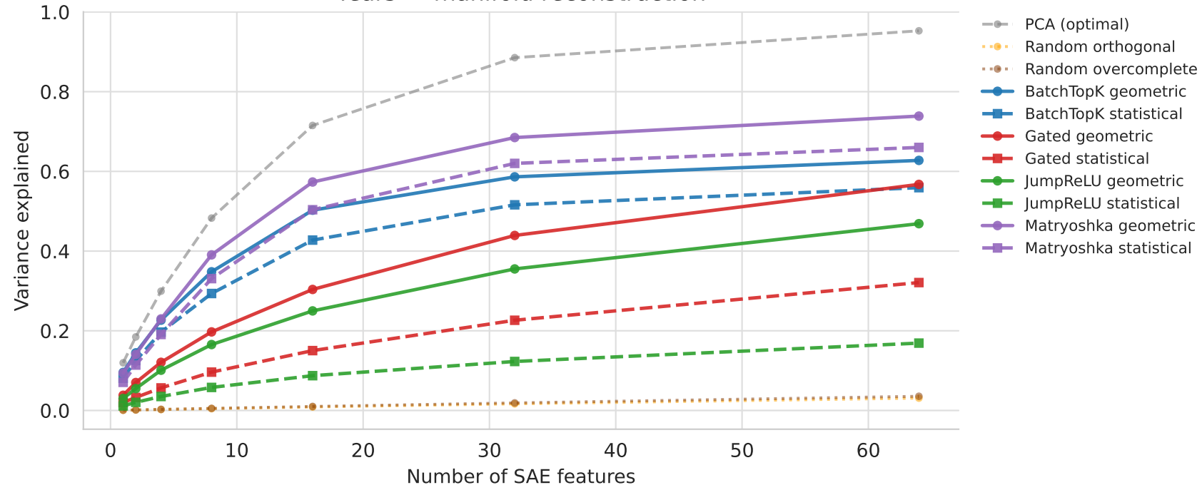
Years — manifold reconstruction
