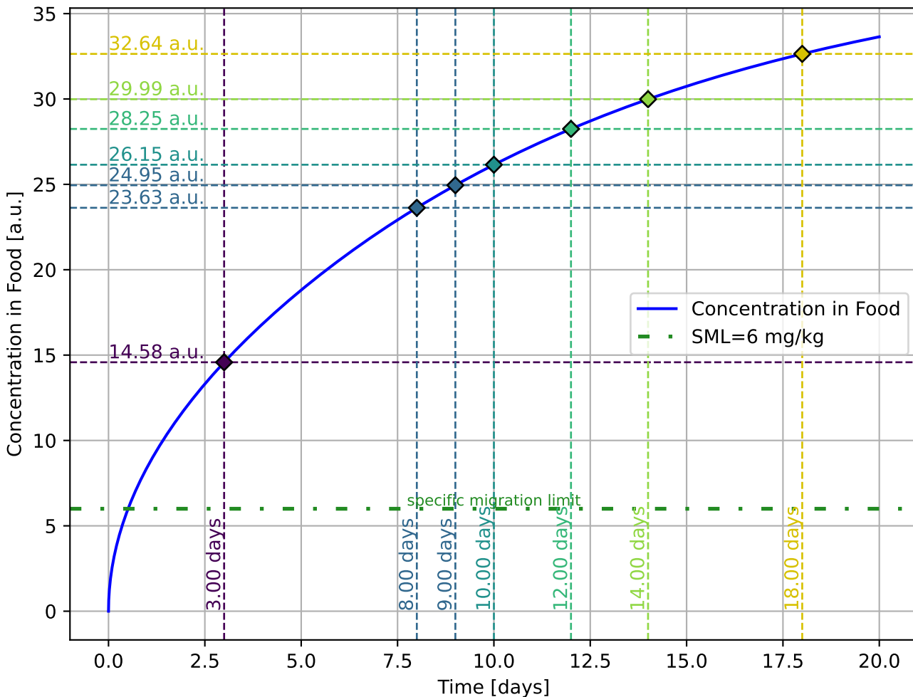
Concentration in Food vs. Time I1076 – LDPE – sandwich
