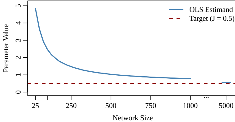
FIGURE 1.—OLS estimator for J across network sizes ( J = 0.5 , h = 1 , d = 1 ); same design as in Table 2(A).
