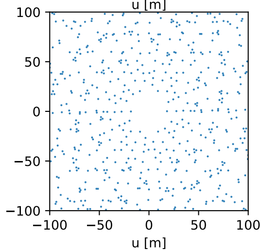
UV Sampling Density
