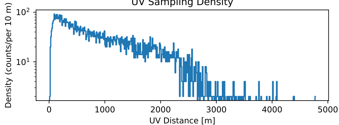
UV Sampling Density
