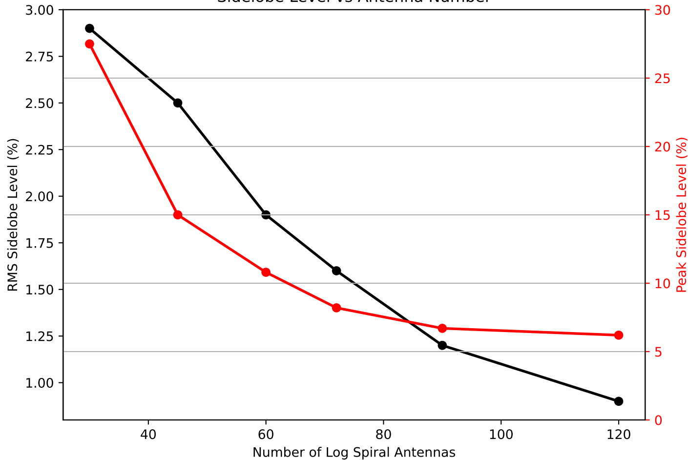
Sidelobe Level vs Antenna Number
