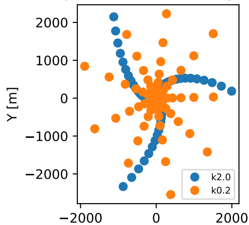
Spiral 90 - Antenna Layout
