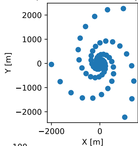
Spiral 90 - Antenna Layout
