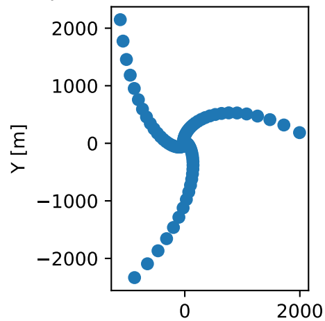
Spiral 90 k=2 - Antenna Layout
