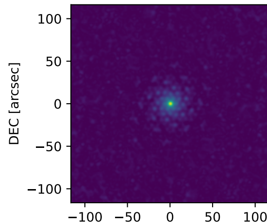
Natural PSF (5.0 GHz)
