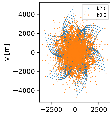
Spiral 90 - UV Coverage
