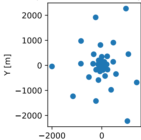
Spiral 45 - Antenna Layout
