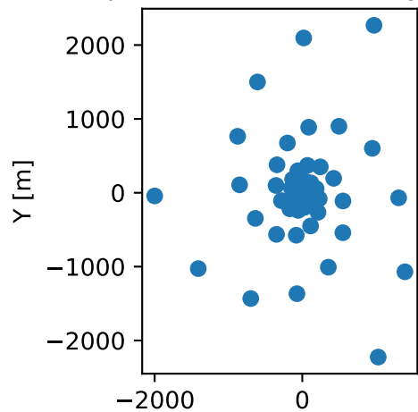
Spiral 60 - Antenna Layout
