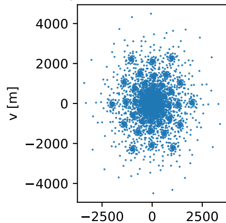
Spiral 60 - UV Coverage
