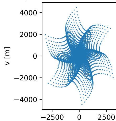
Spiral 90 k=2 - UV Coverage
