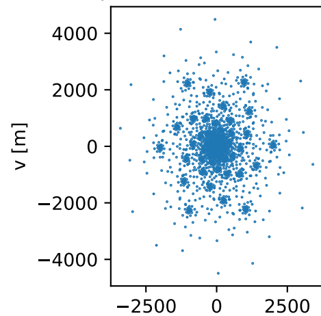
Spiral 45 - UV Coverage
