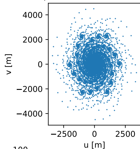
Spiral 90 - UV Coverage
