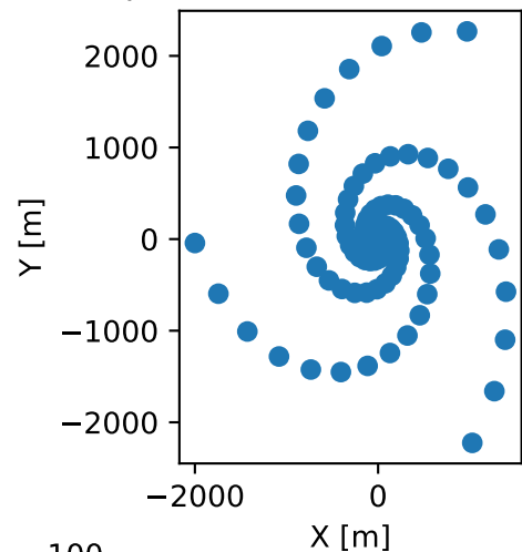
Spiral 120 - Antenna Layout
