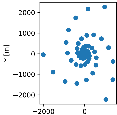
Spiral 72 - Antenna Layout
