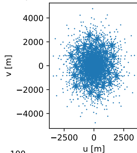
Spiral 90 k=0.2 - UV Coverage
