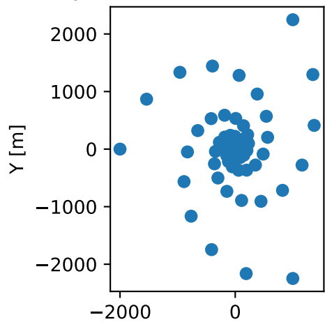
Hybrid 120 - Antenna Layout
