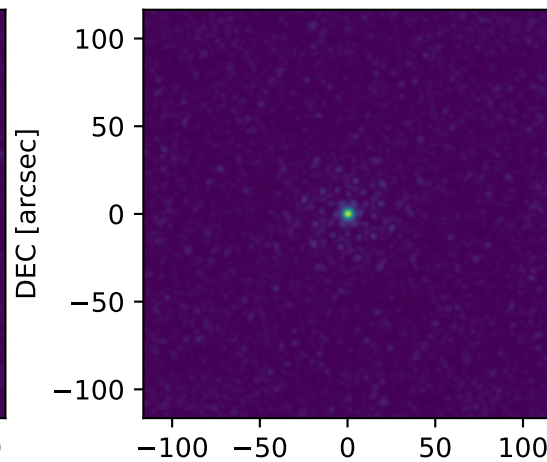
Uniform PSF (5.0 GHz)
