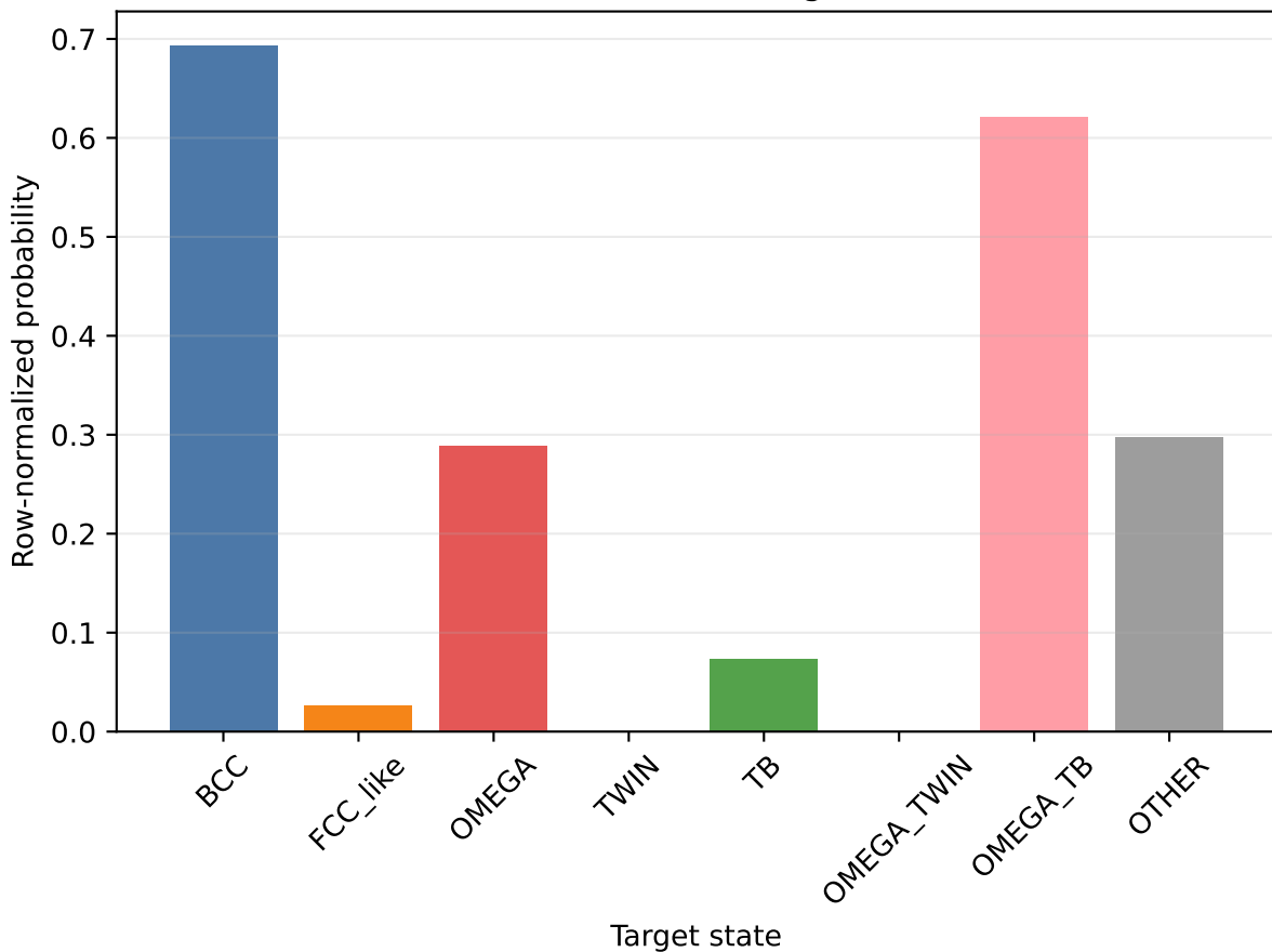
Ti20Nb: transitions from omega-related states
