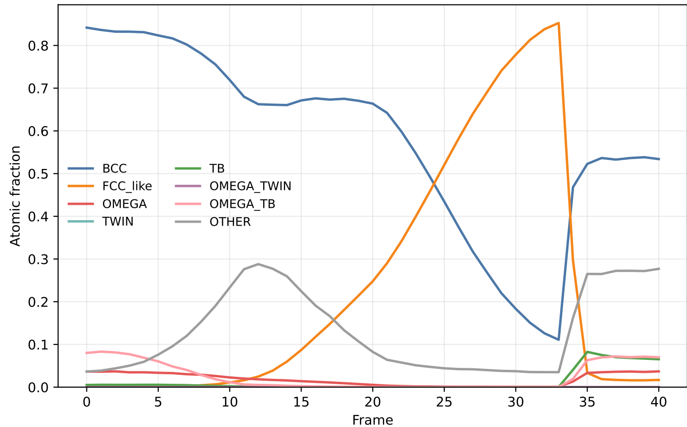
Ti20Nb: state fraction evolution
