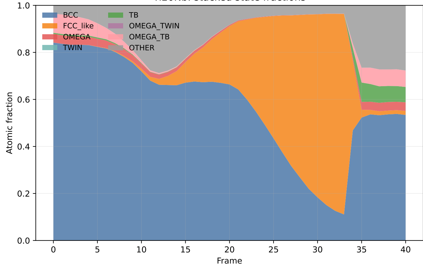
Ti20Nb: stacked state fractions
