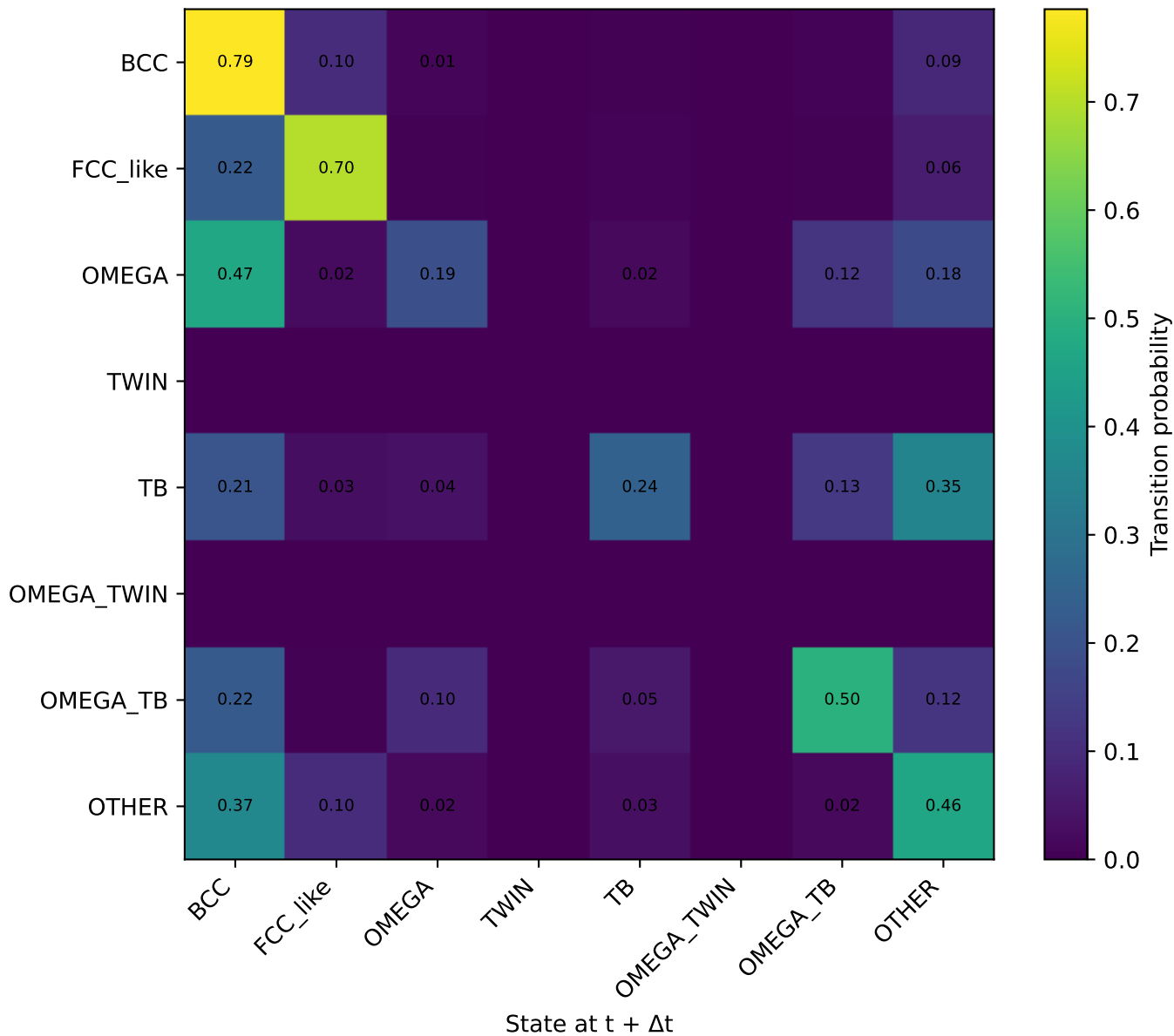
Ti20Nb: row-normalized transition matrix
