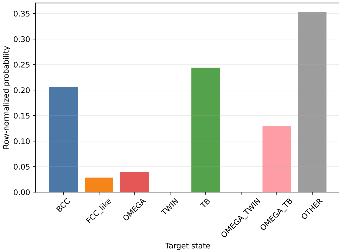
Ti20Nb: transitions from twin/TB states
