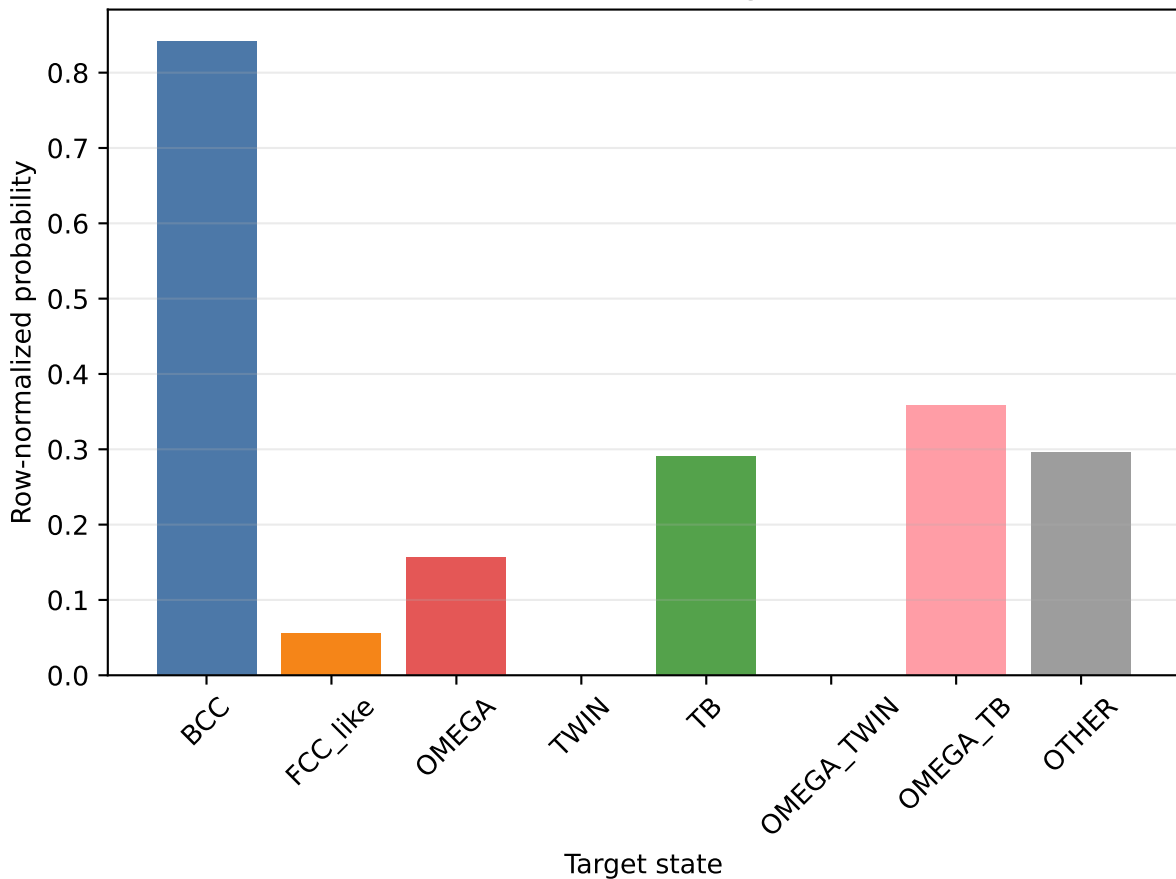
Ti30Nb: transitions from omega-related states
