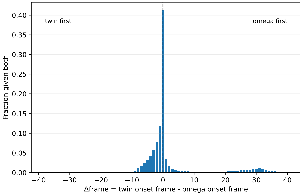
Ti30Nb: omega-twin onset lag distribution
