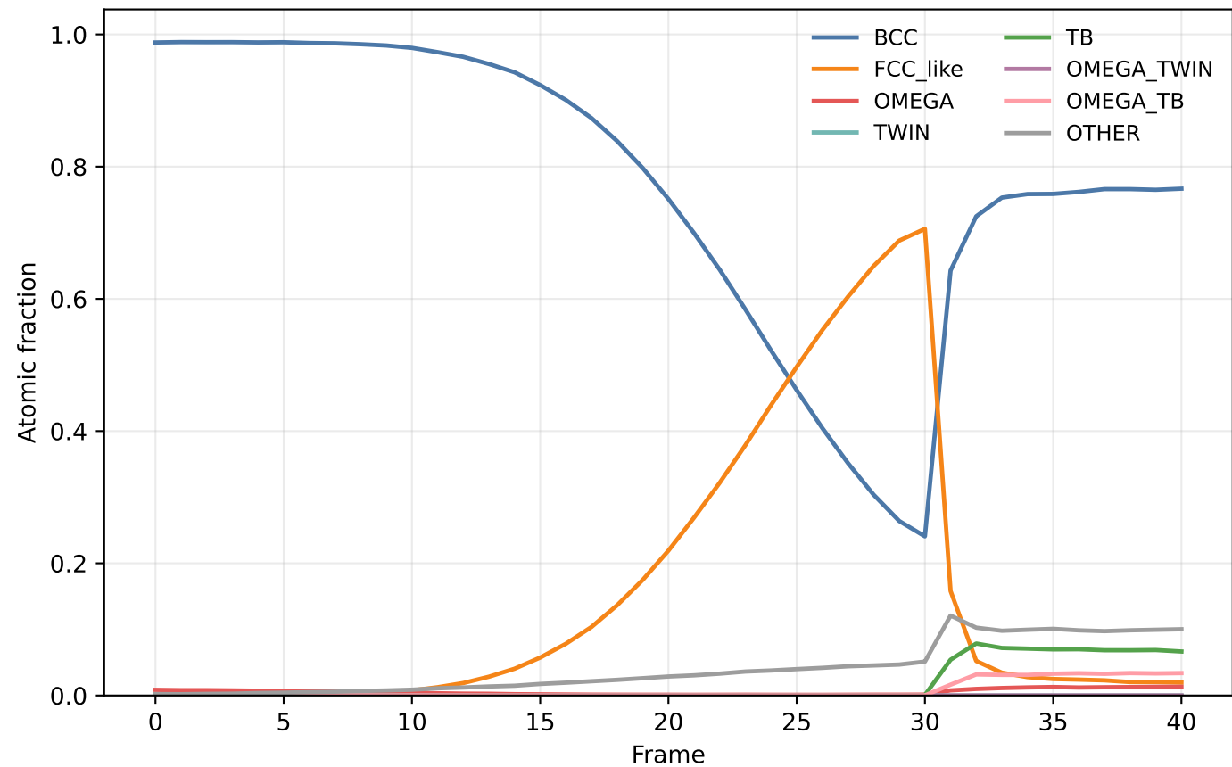
Ti30Nb: state fraction evolution
