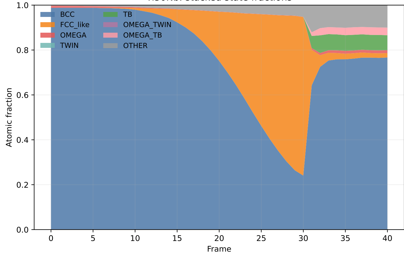
Ti30Nb: stacked state fractions
