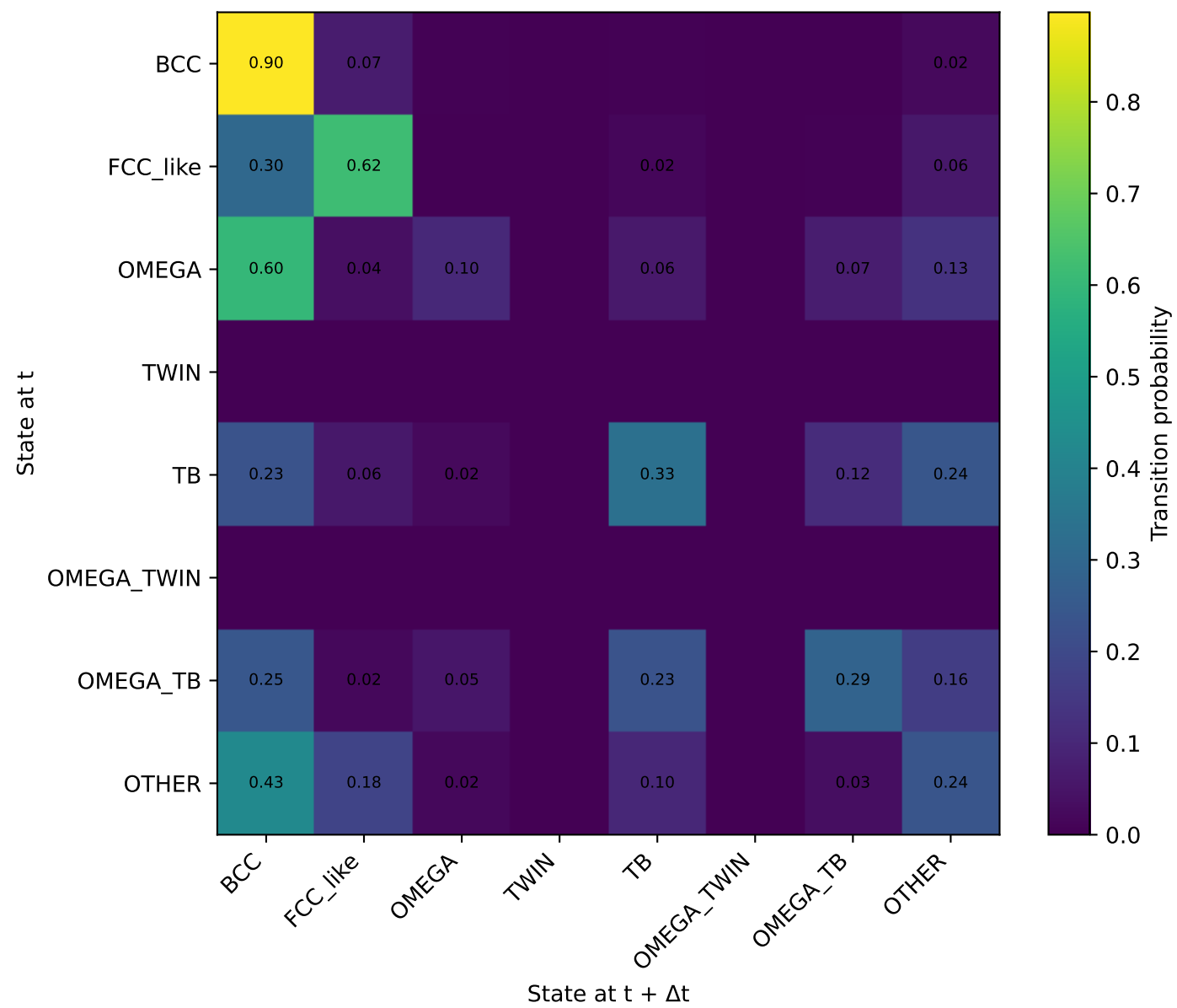
Ti30Nb: row-normalized transition matrix
