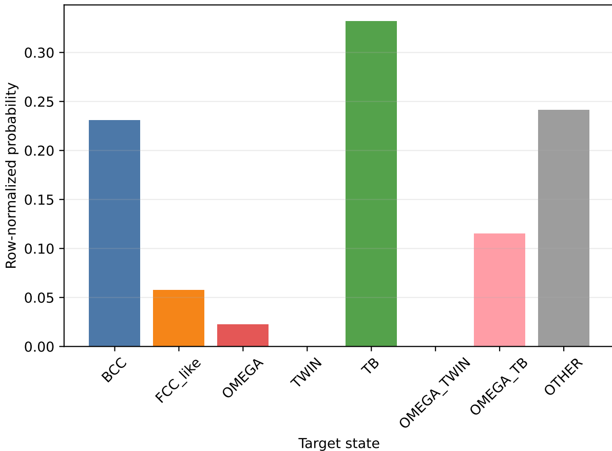
Ti30Nb: transitions from twin/TB states
