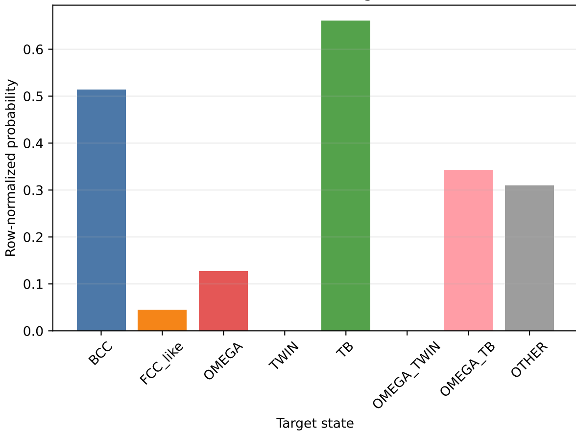
Ti40Nb: transitions from omega-related states
