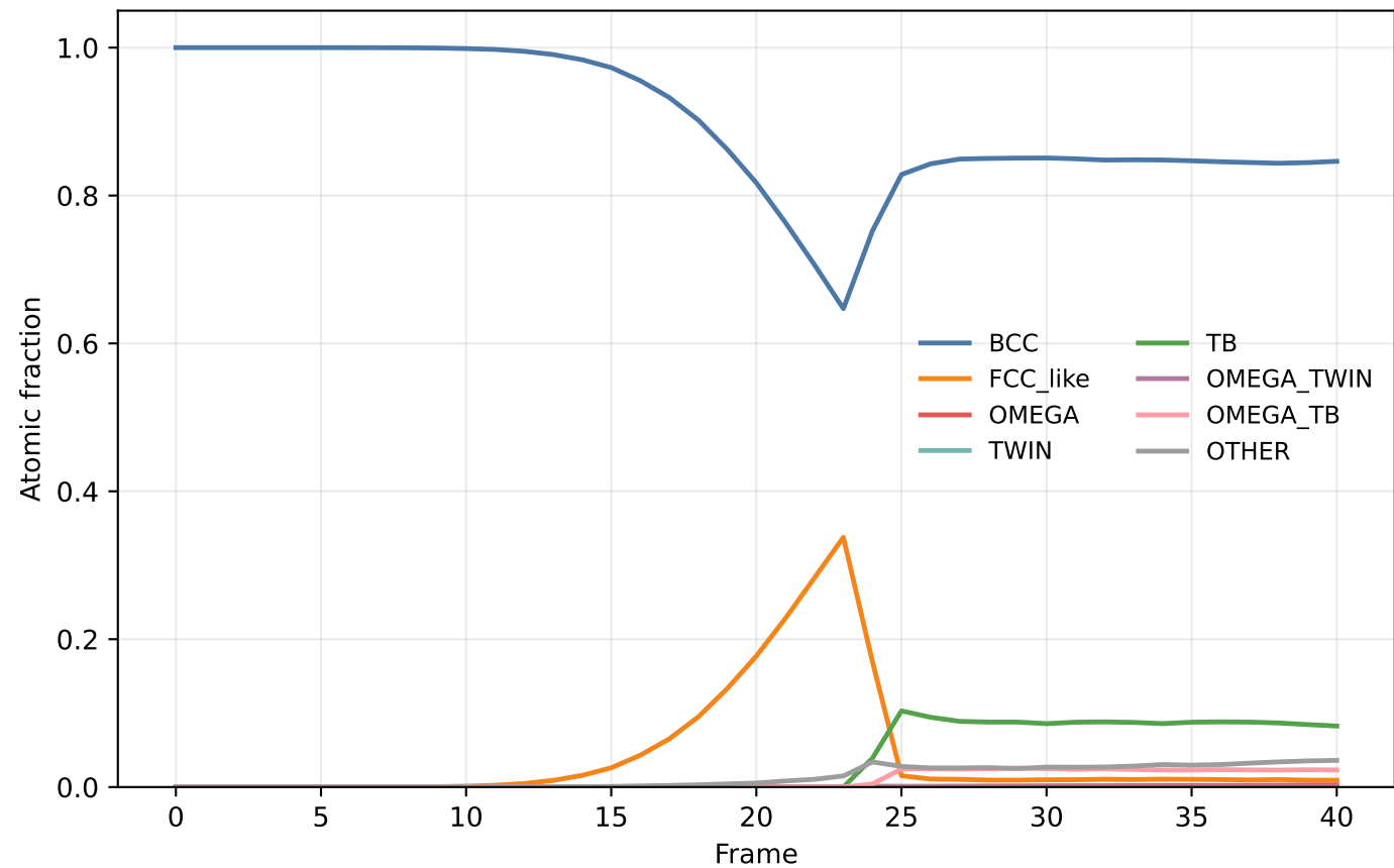
Ti40Nb: state fraction evolution
