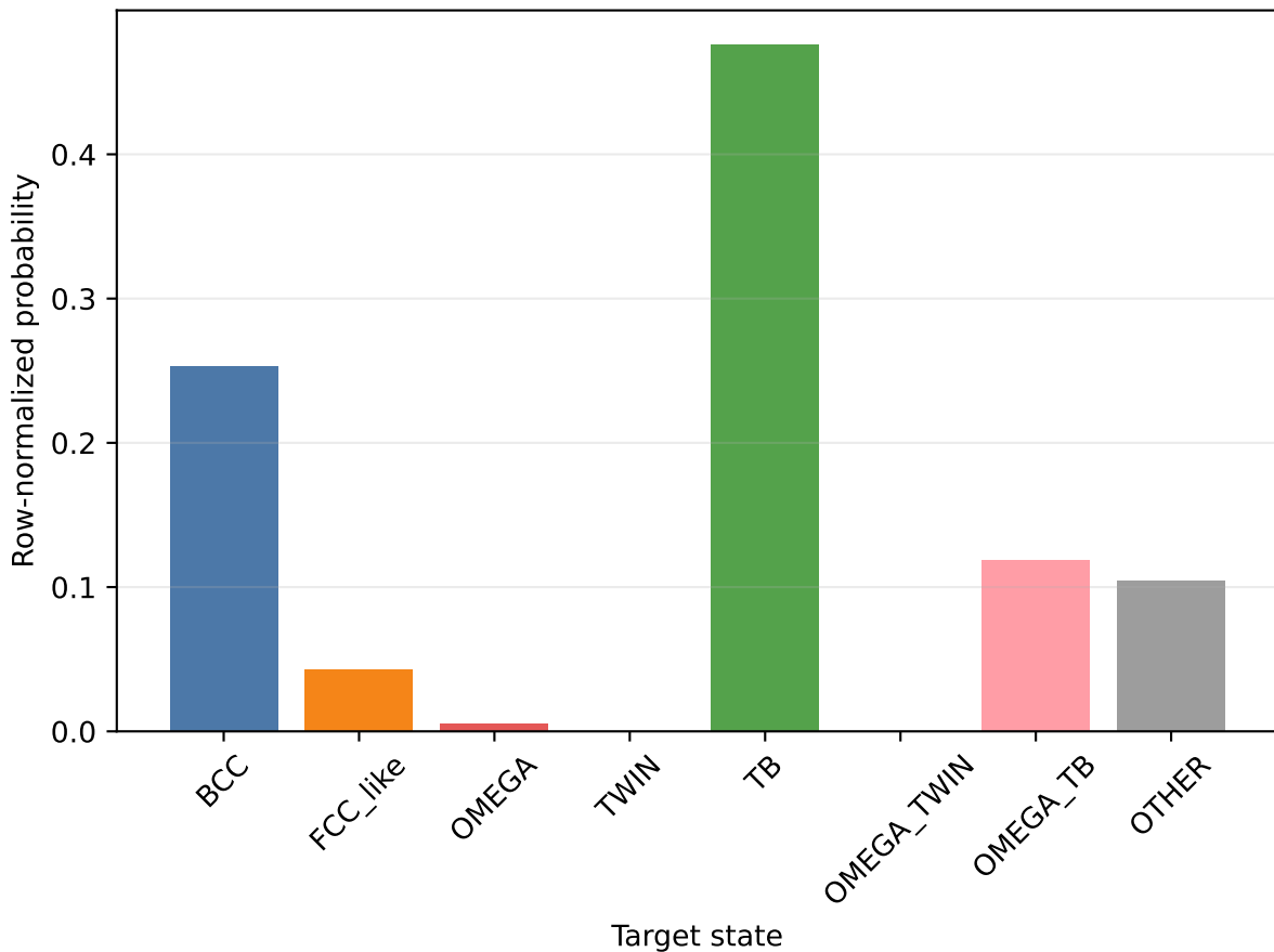
Ti40Nb: transitions from twin/TB states
