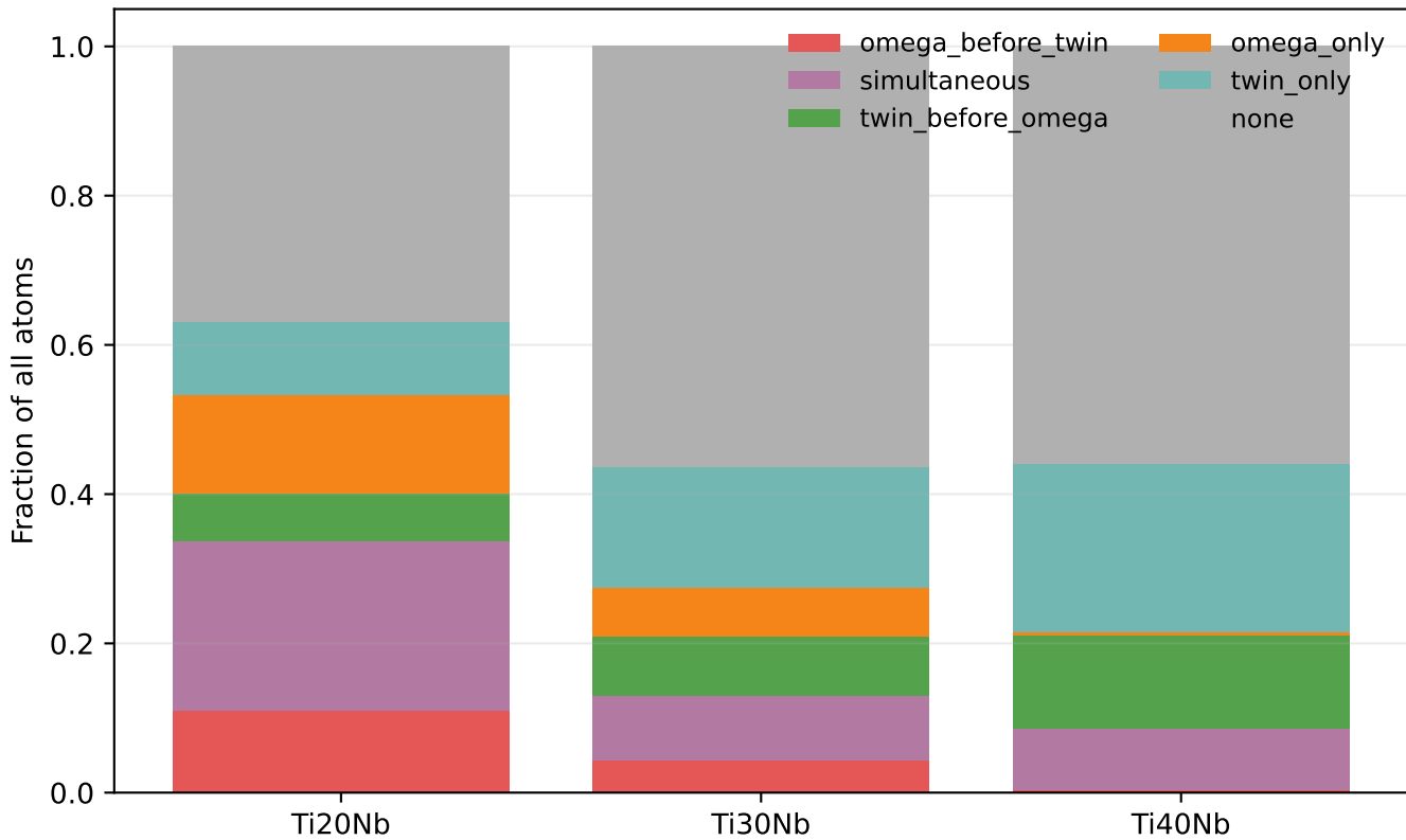
Omega-twin onset class summary
