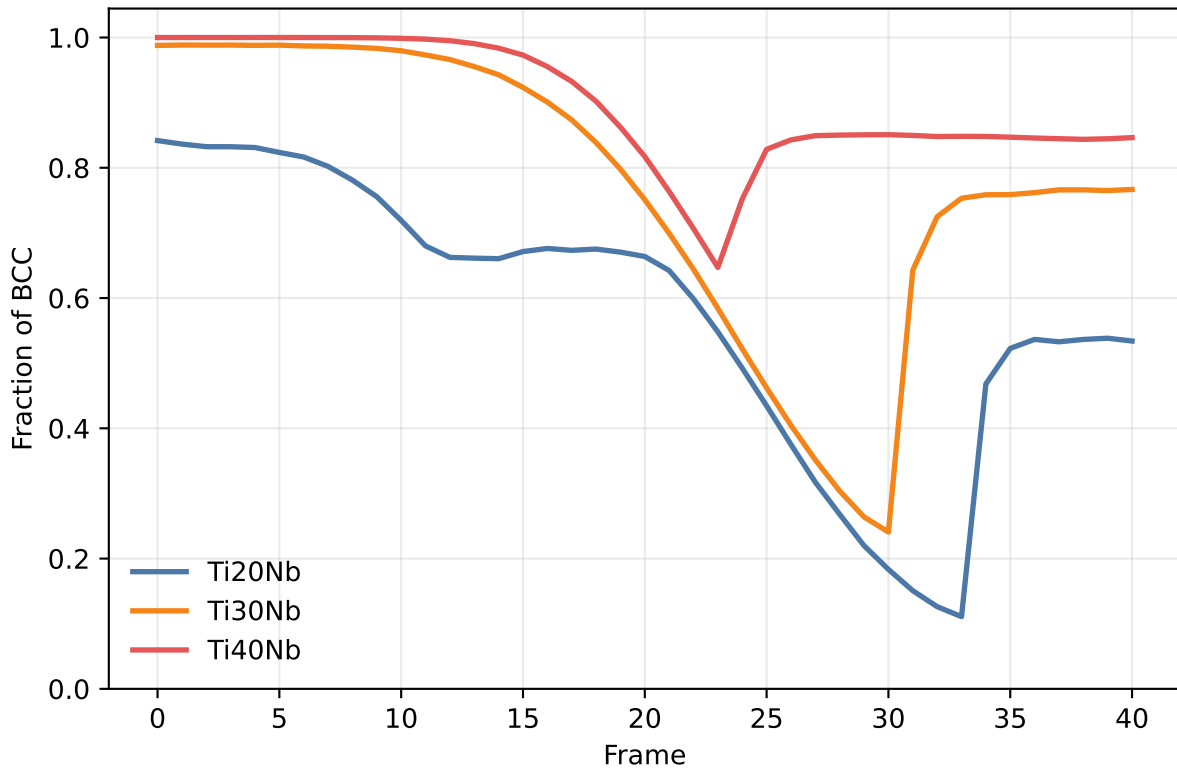
Composition dependence of BCC
