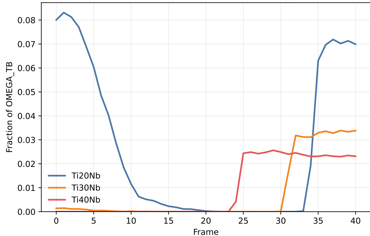
Composition dependence of OMEGA_TB
