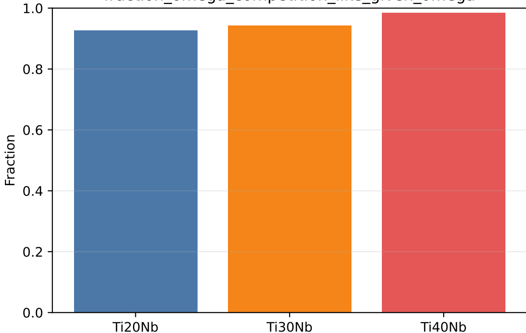
fraction_omega_competition_like_given_omega
