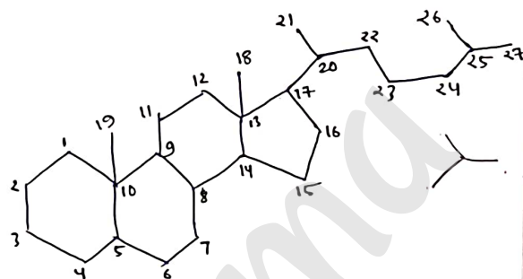
cholesterol (C-27)
