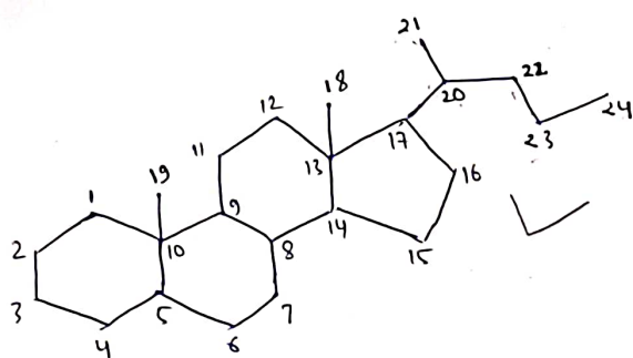
cholan (C-24)
