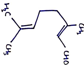
Citral-a (geranial)
