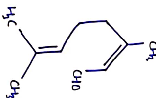
Citral-b (neral)
