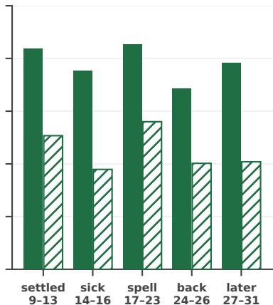
survival-time model
